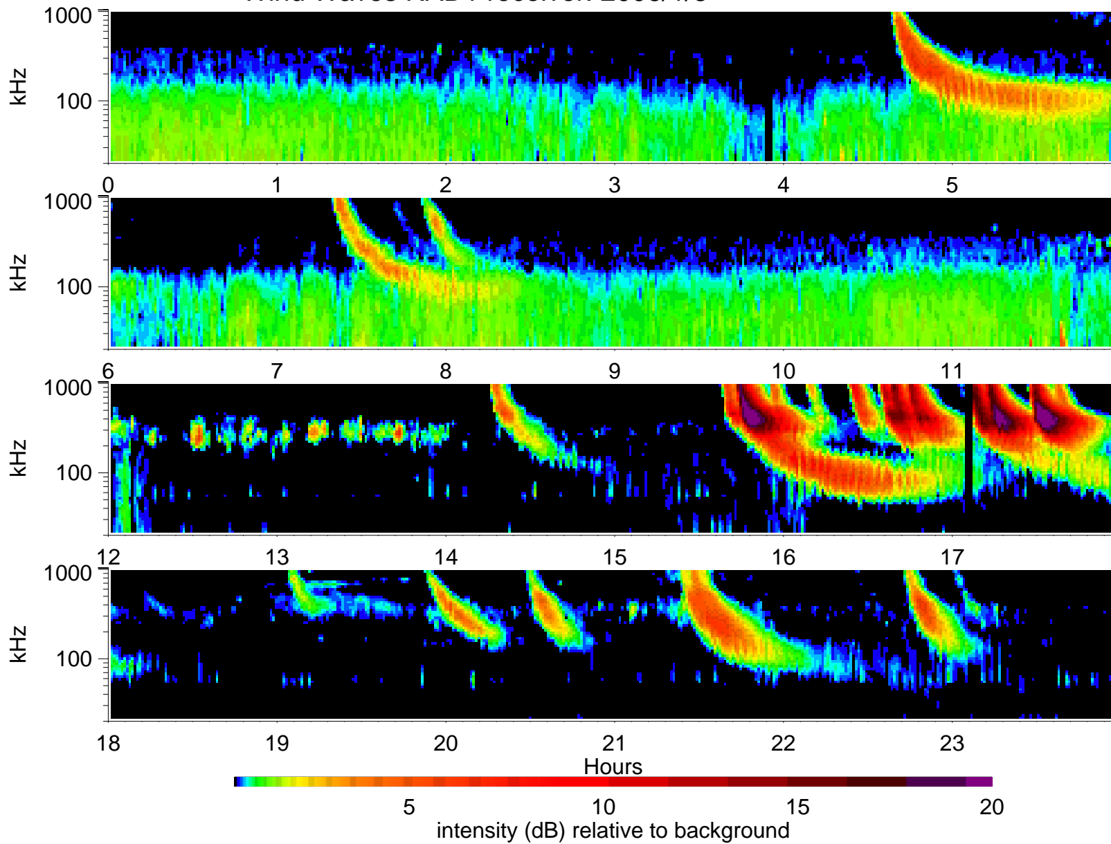
Wind Waves RAD1 receiver: 2006/1/3
