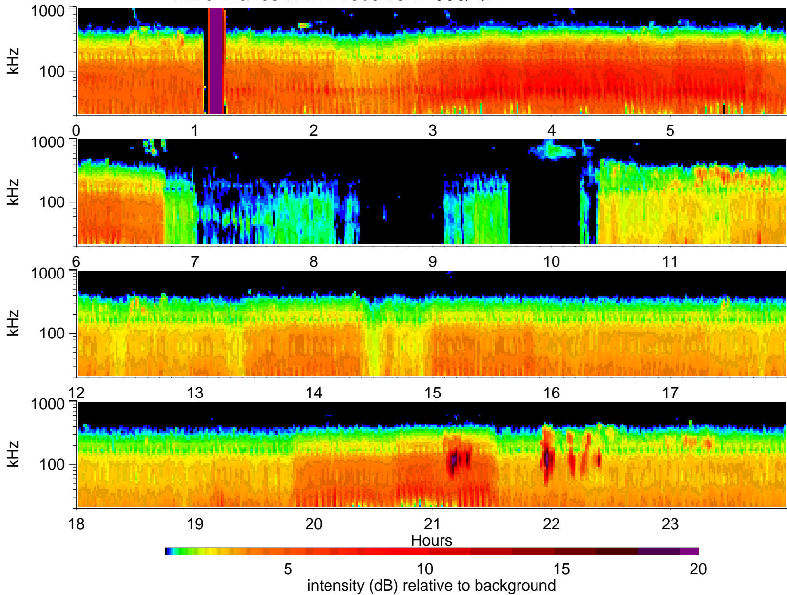
Wind Waves RAD1 receiver: 2006/1/2
