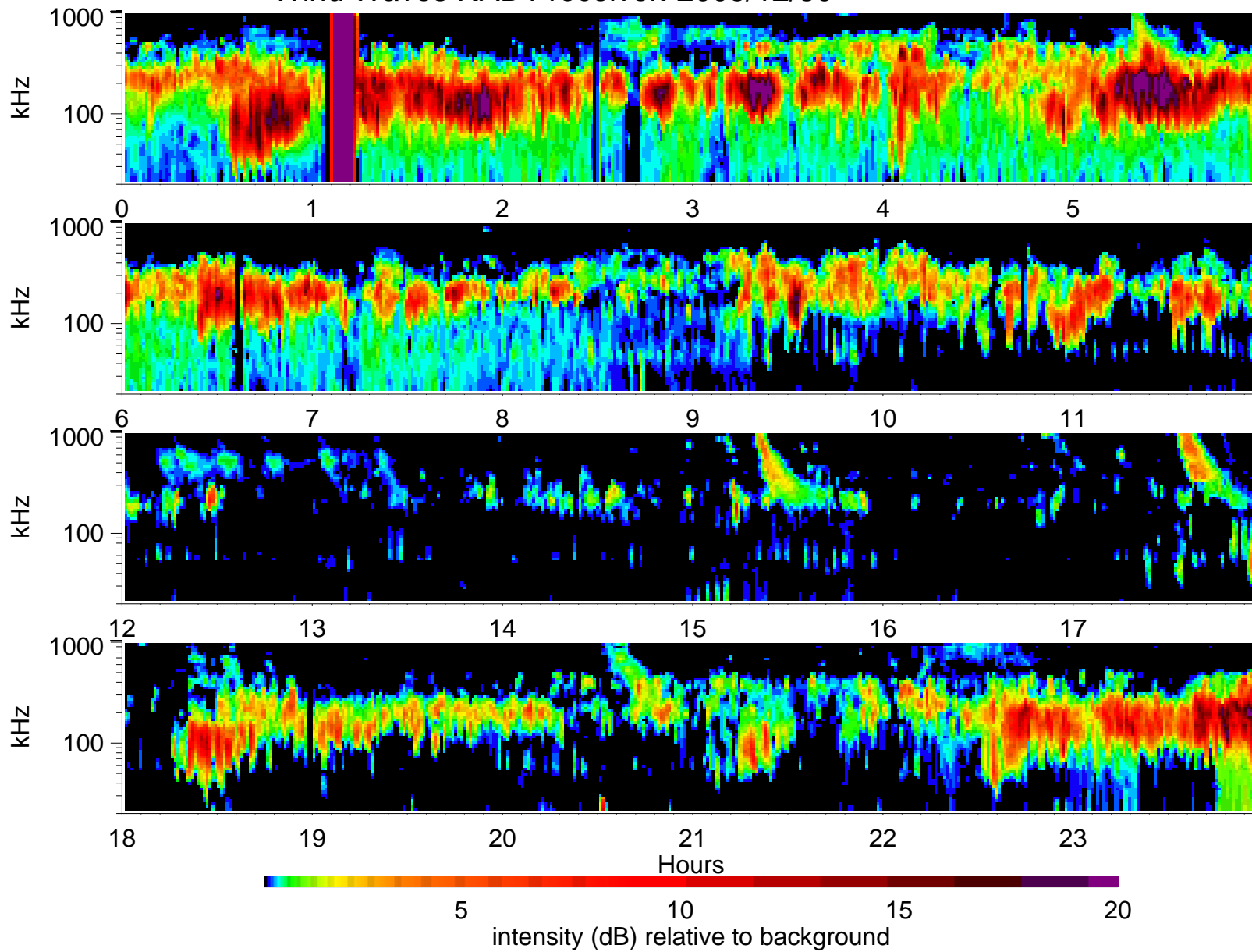
Wind Waves RAD1 receiver: 2005/12/30
