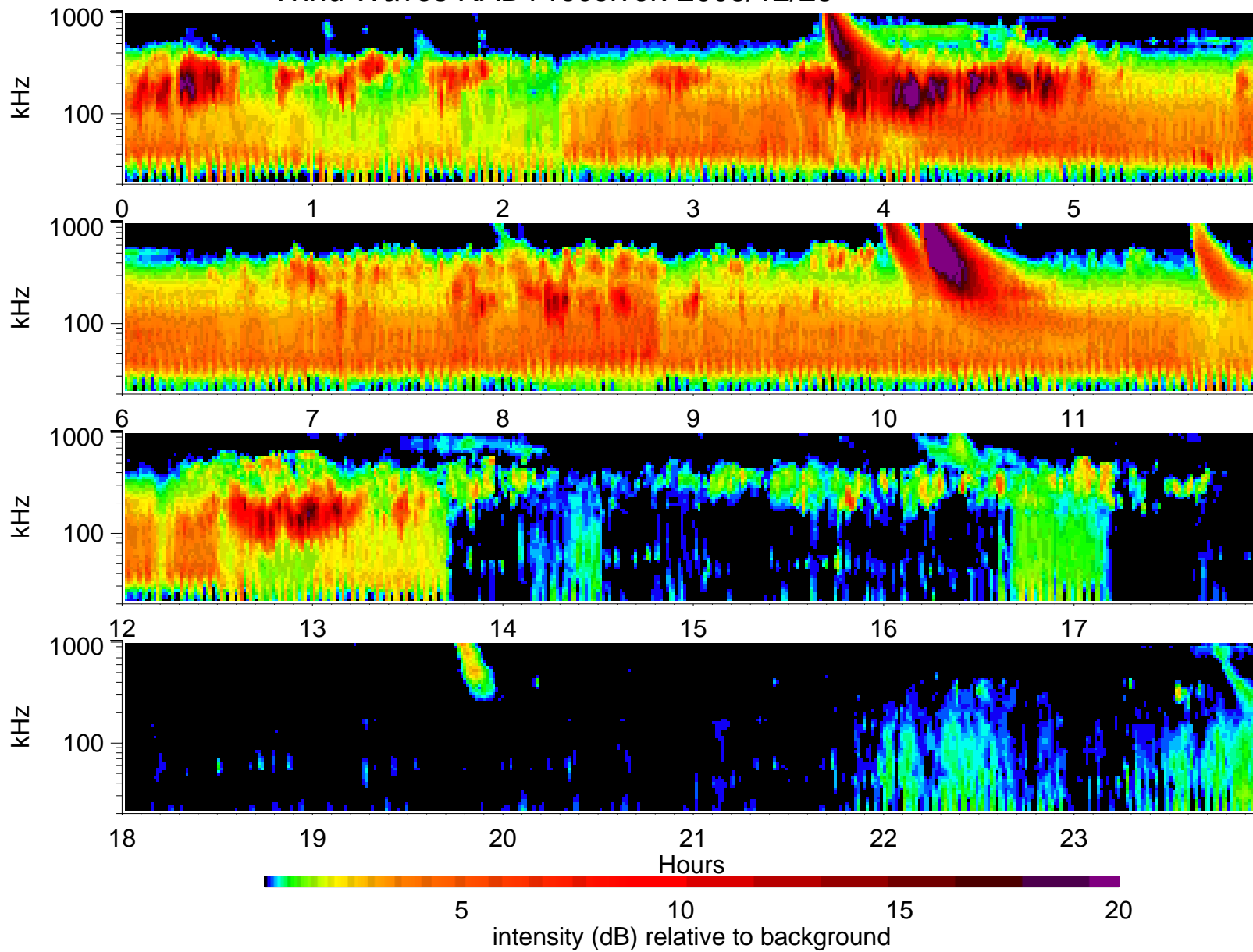
Wind Waves RAD1 receiver: 2005/12/25
