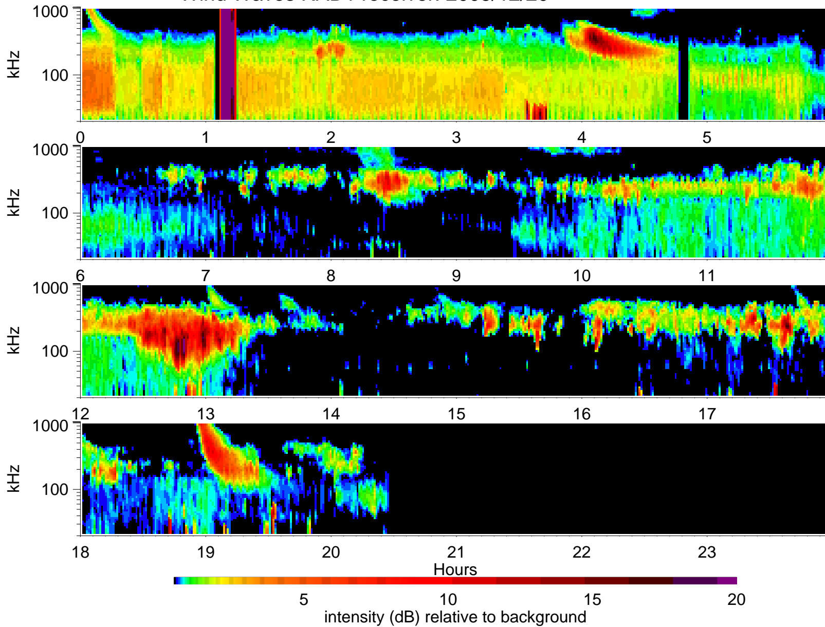
Wind Waves RAD1 receiver: 2005/12/20
