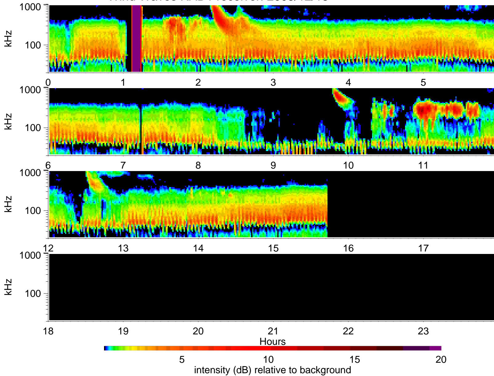
Wind Waves RAD1 receiver: 2005/12/18
