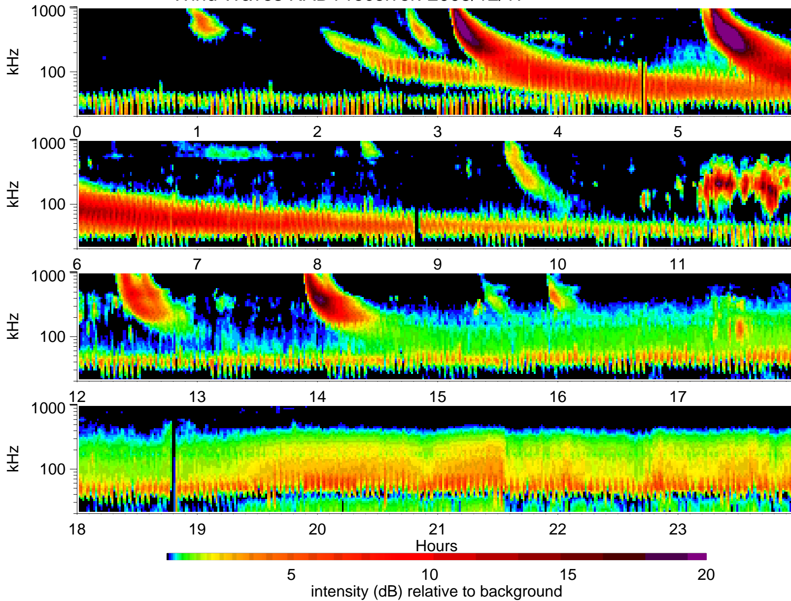
Wind Waves RAD1 receiver: 2005/12/17
