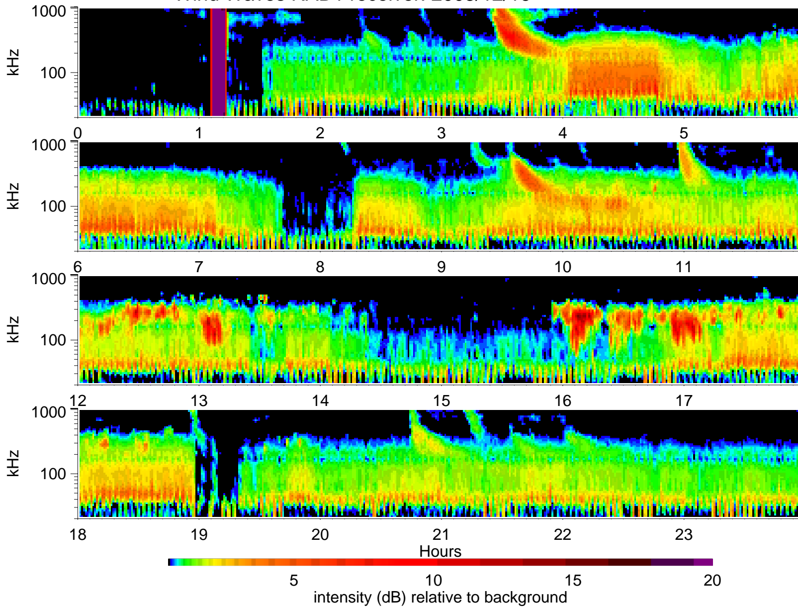
Wind Waves RAD1 receiver: 2005/12/16
