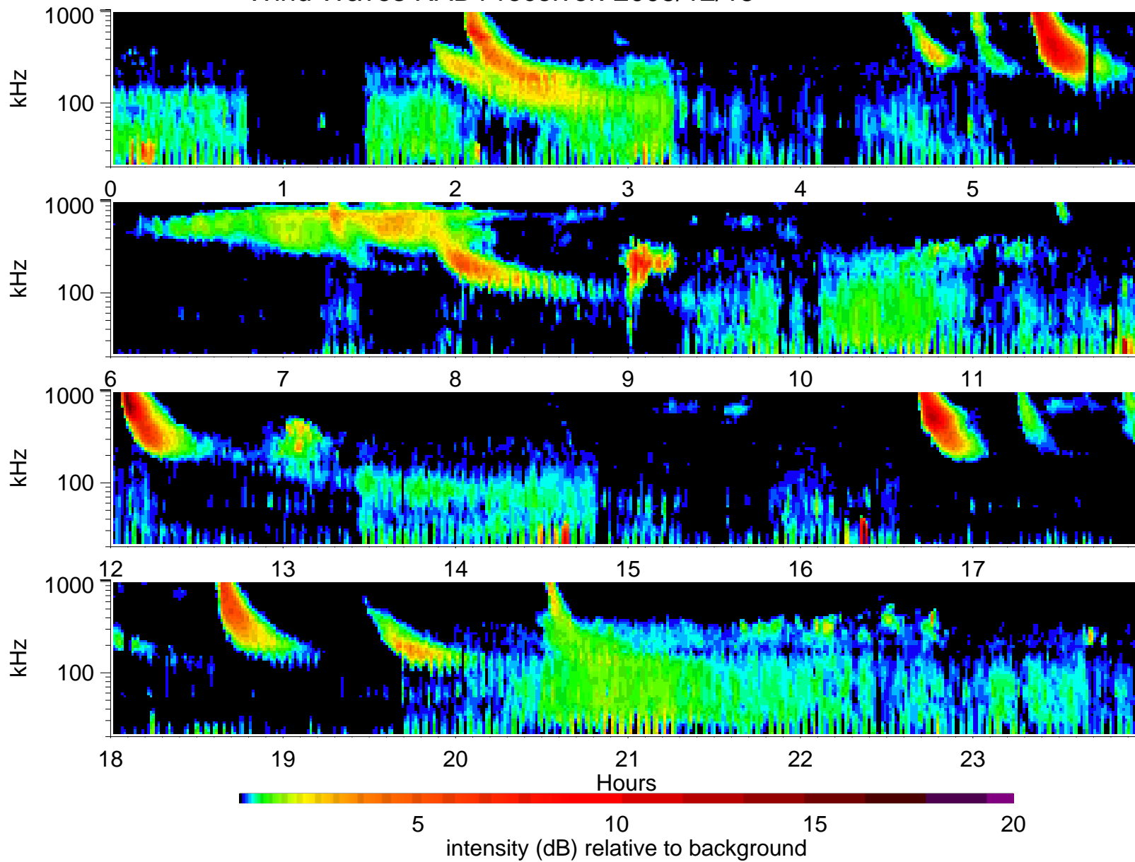
Wind Waves RAD1 receiver: 2005/12/15
