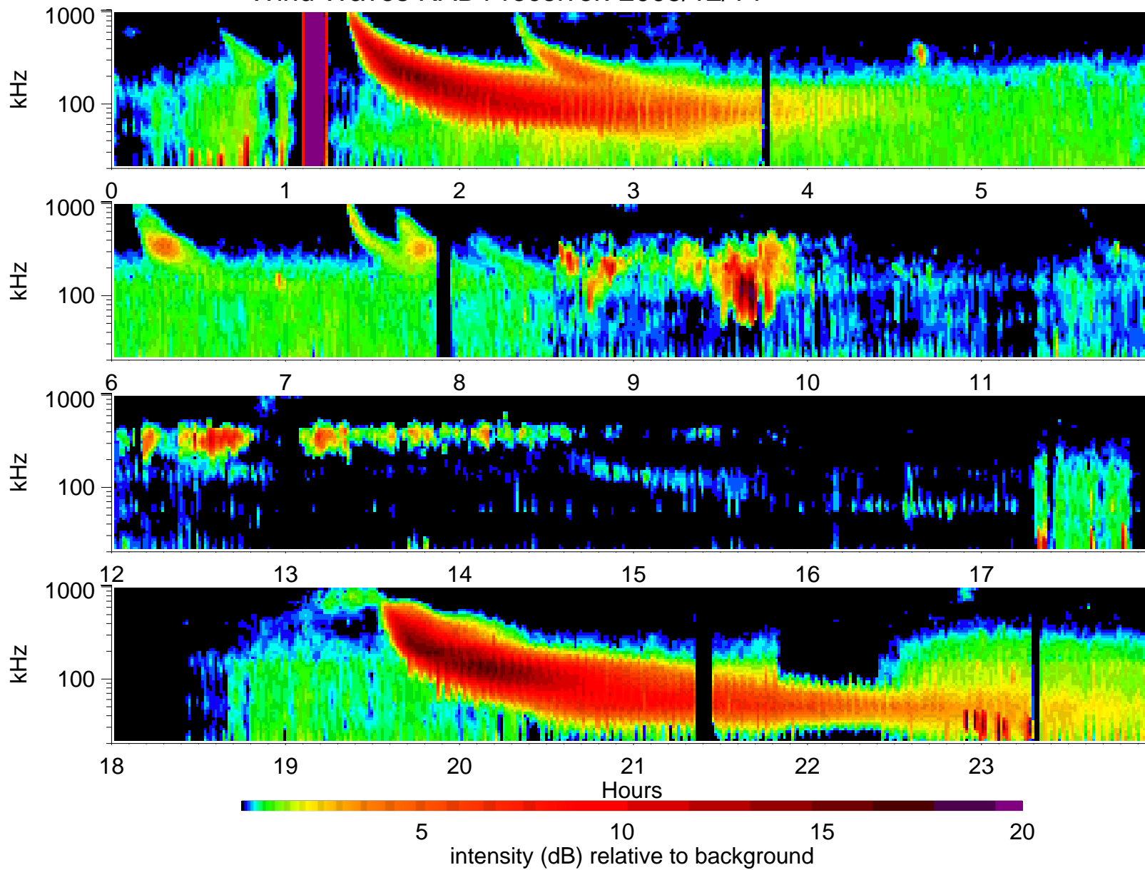
Wind Waves RAD1 receiver: 2005/12/14
