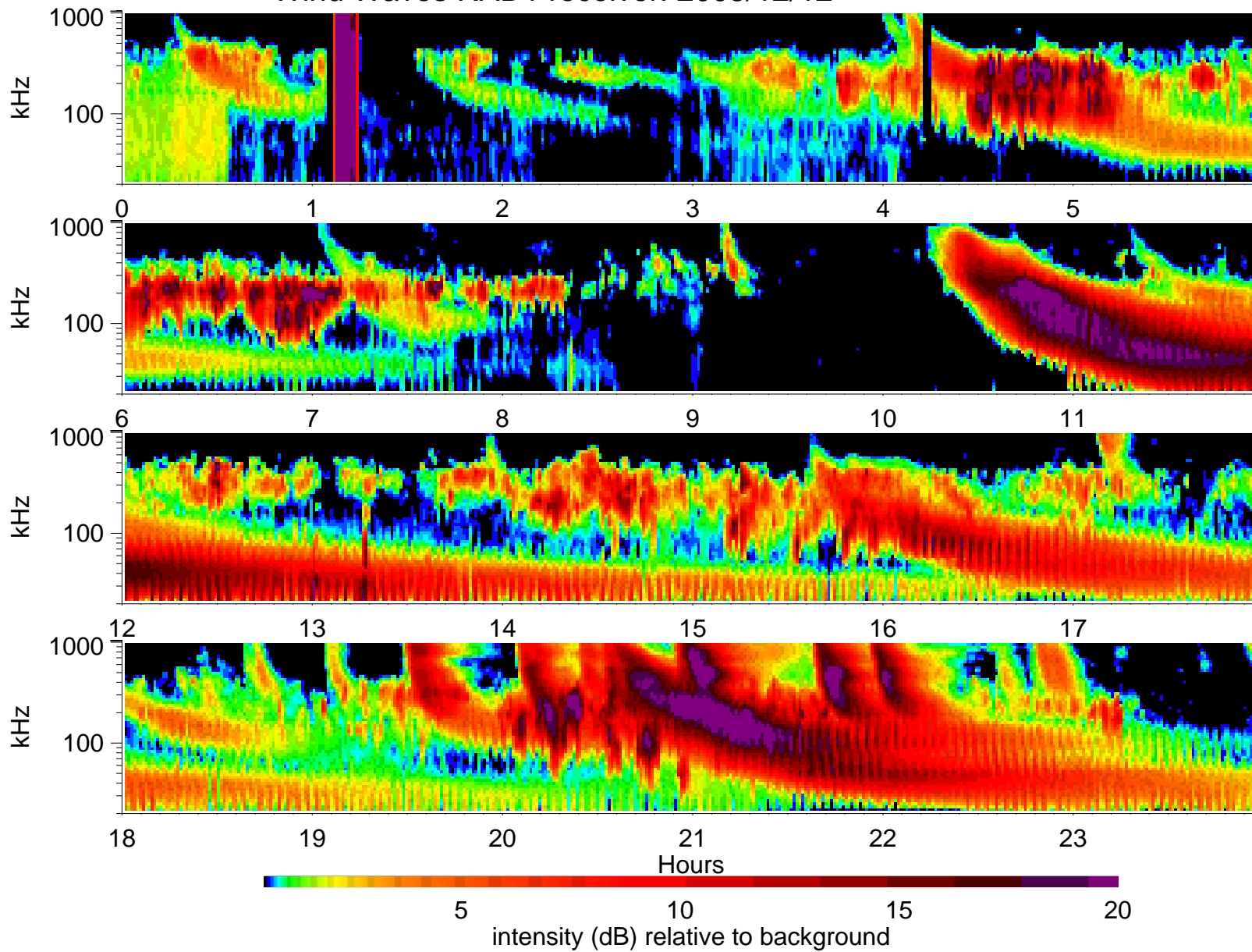
Wind Waves RAD1 receiver: 2005/12/12
