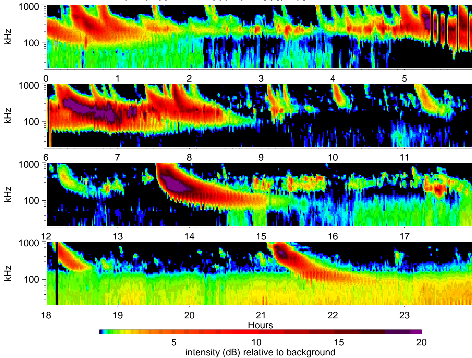
Wind Waves RAD1 receiver: 2005/12/5
