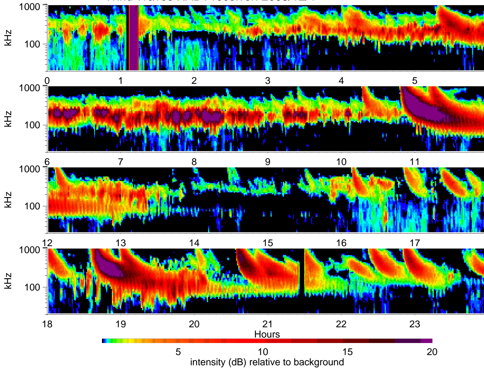
Wind Waves RAD1 receiver: 2005/12/4
