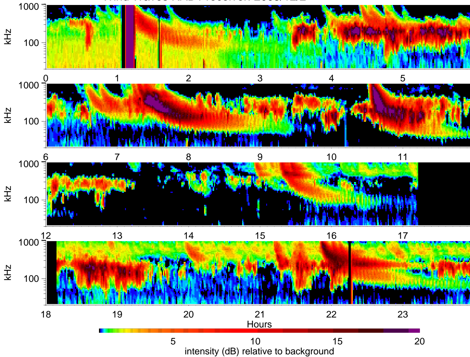
Wind Waves RAD1 receiver: 2005/12/2
