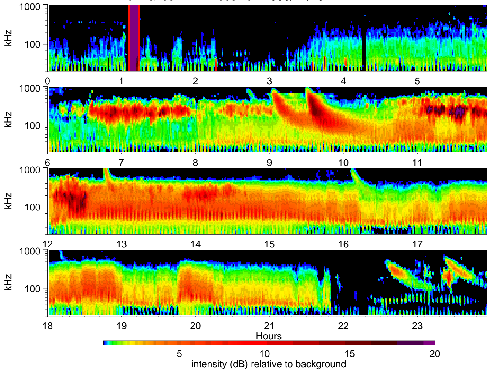
Wind Waves RAD1 receiver: 2005/11/28
