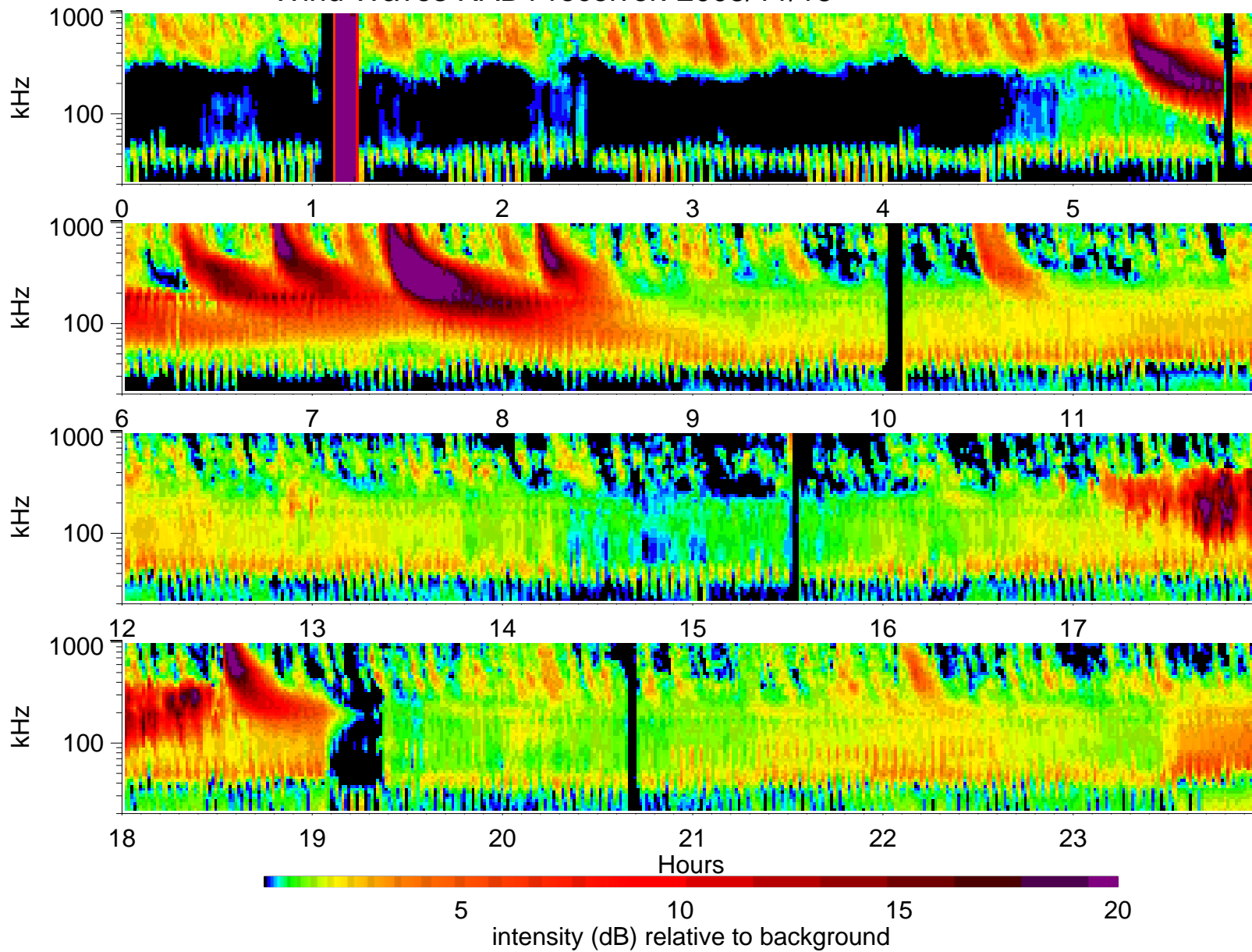
Wind Waves RAD1 receiver: 2005/11/18
