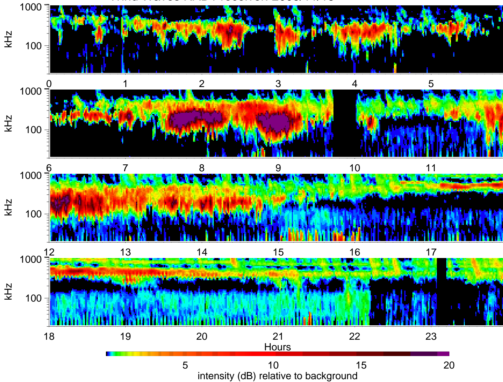
Wind Waves RAD1 receiver: 2005/11/15
