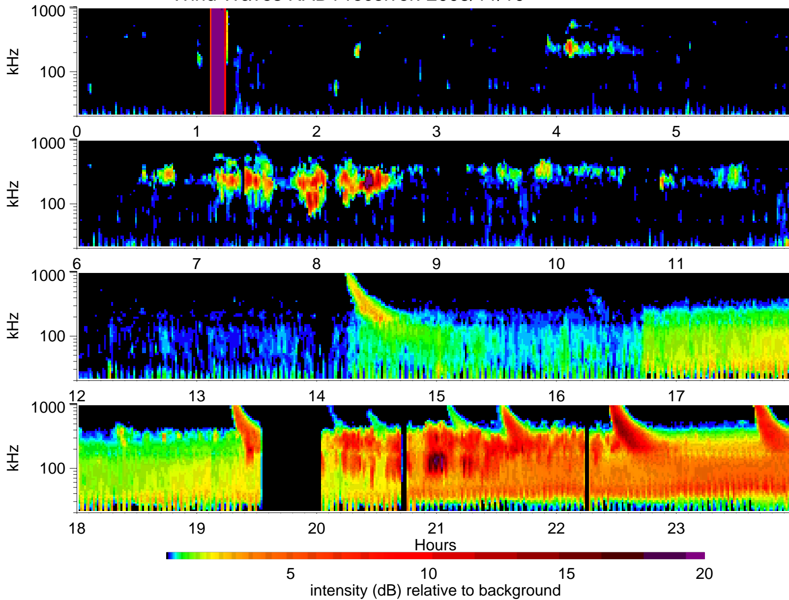
Wind Waves RAD1 receiver: 2005/11/10
