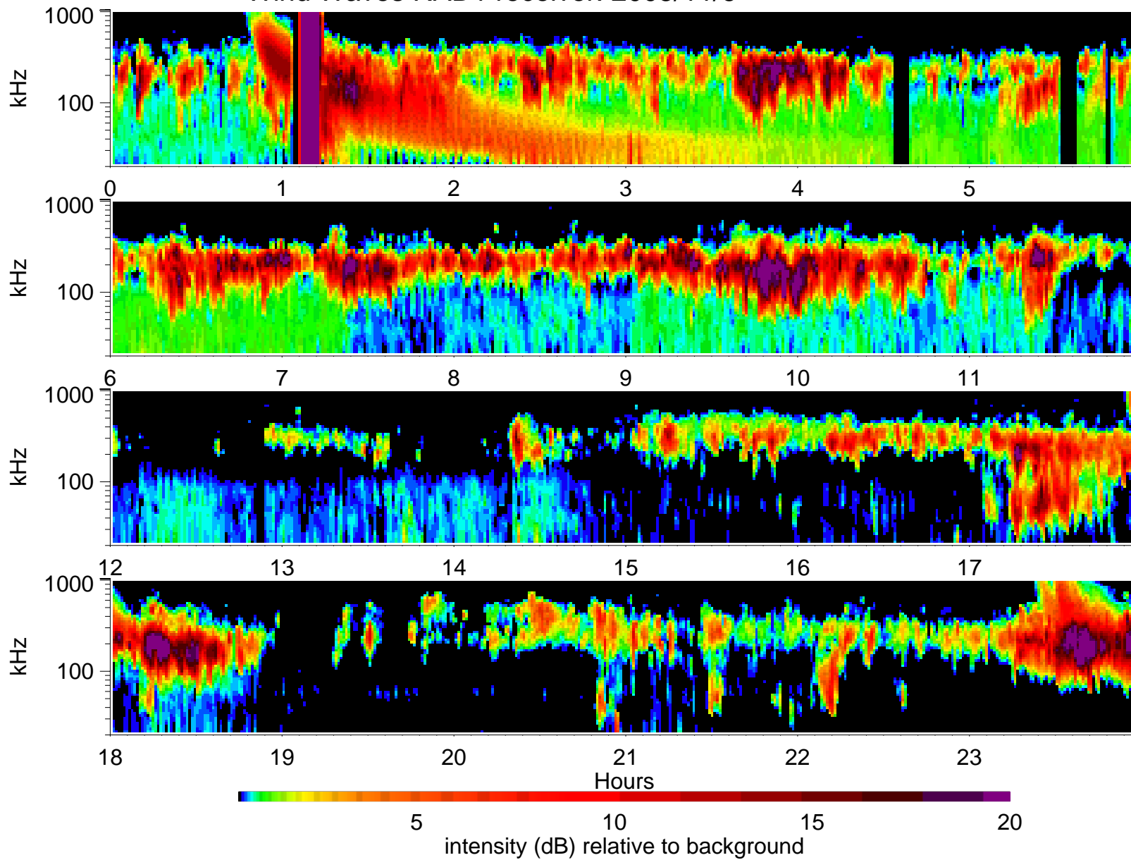
Wind Waves RAD1 receiver: 2005/11/6
