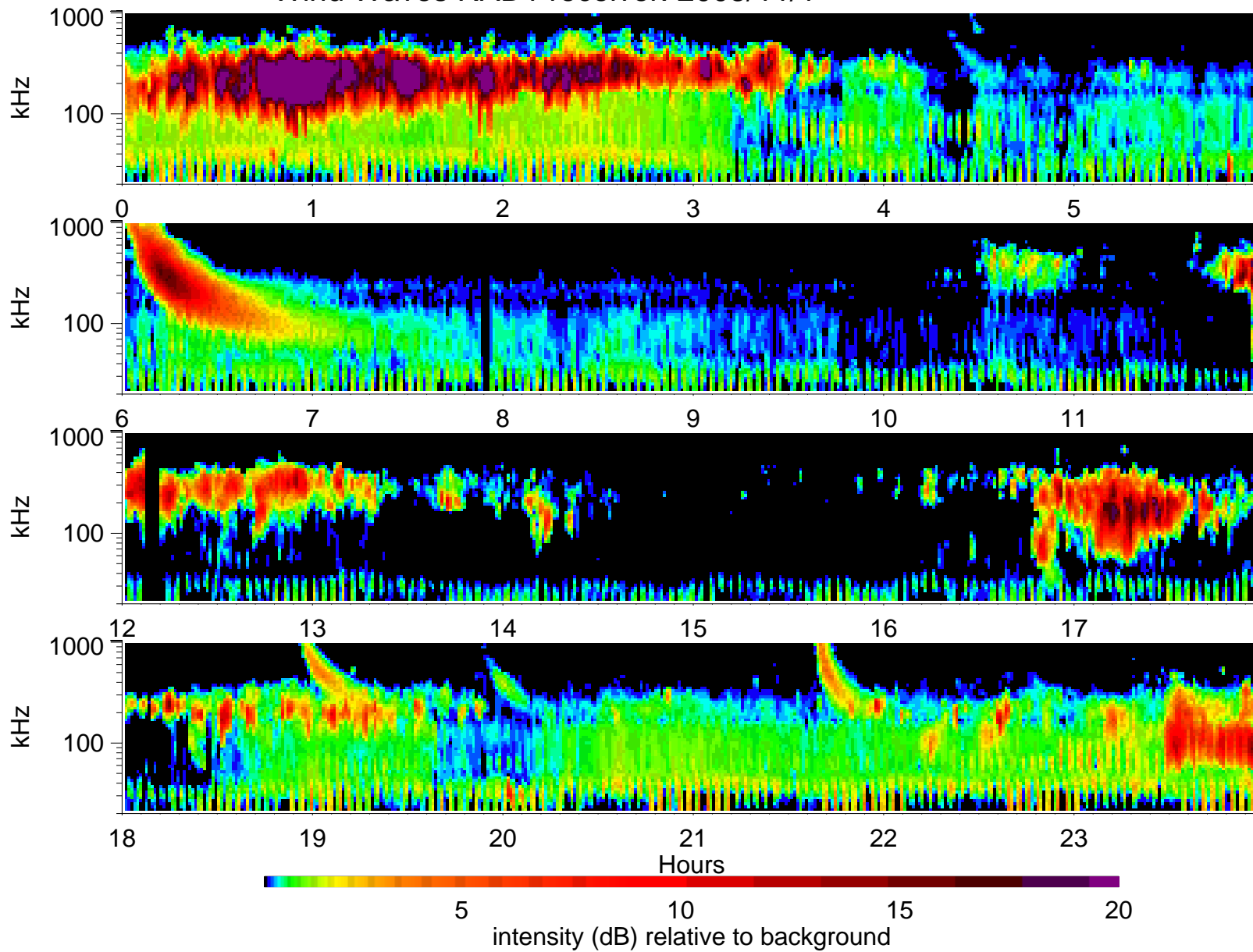
Wind Waves RAD1 receiver: 2005/11/1
