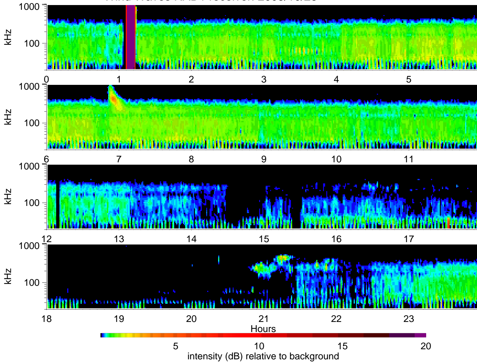
Wind Waves RAD1 receiver: 2005/10/23
