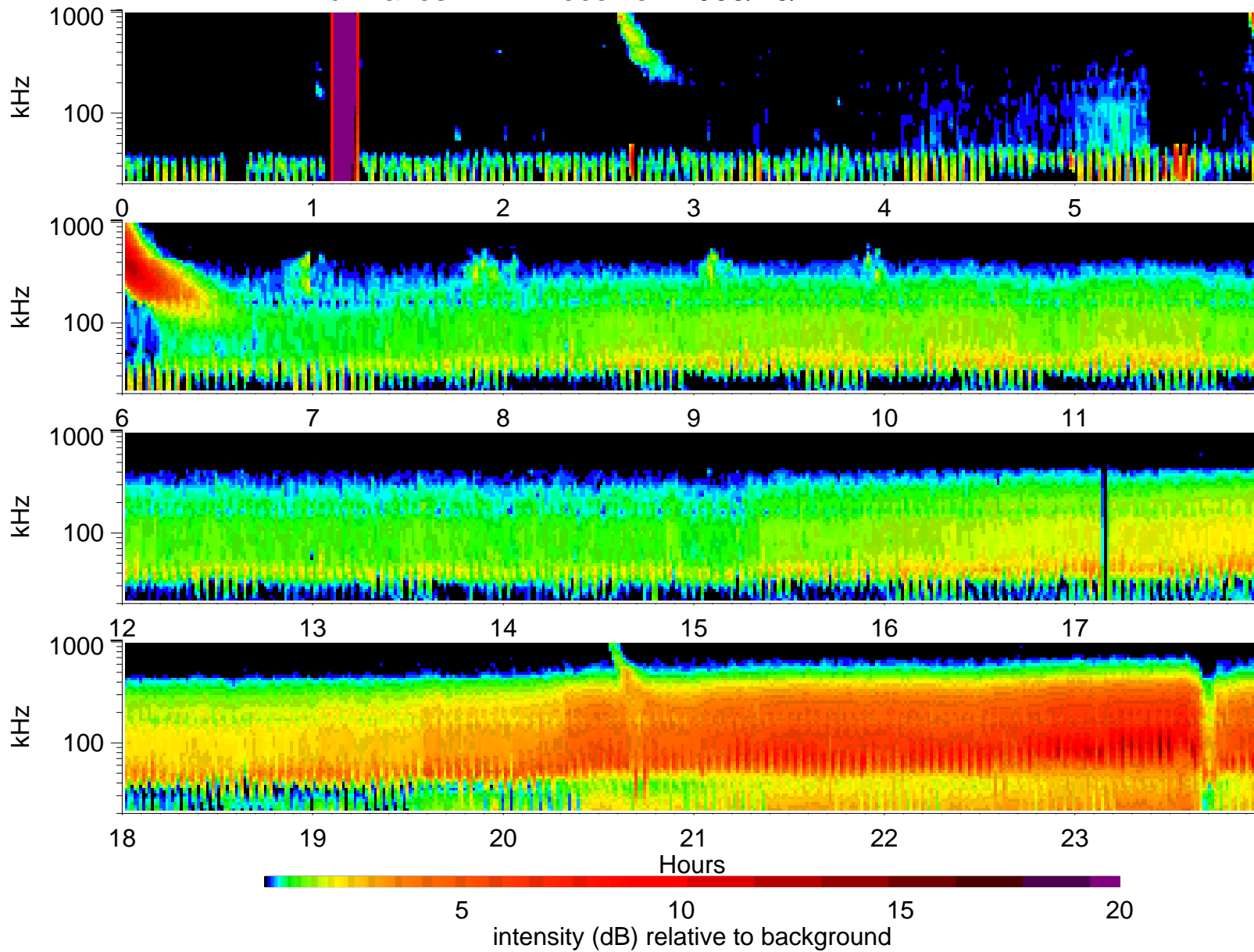
Wind Waves RAD1 receiver: 2005/10/21
