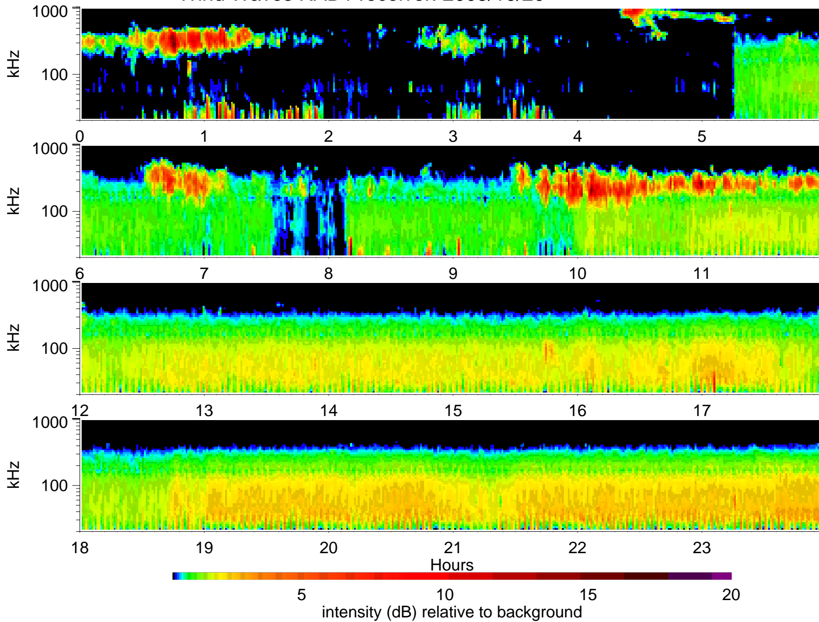
Wind Waves RAD1 receiver: 2005/10/20
