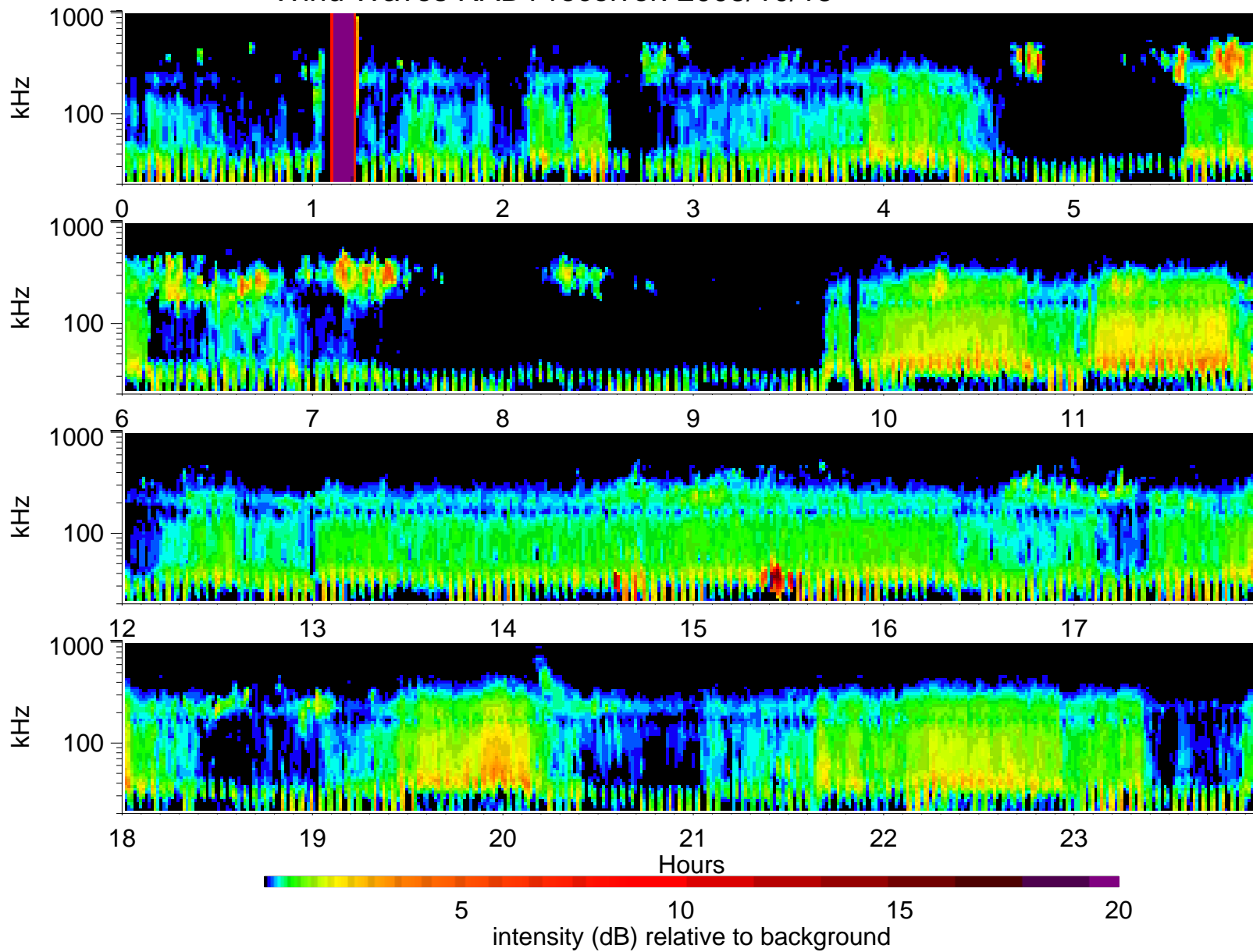
Wind Waves RAD1 receiver: 2005/10/15
