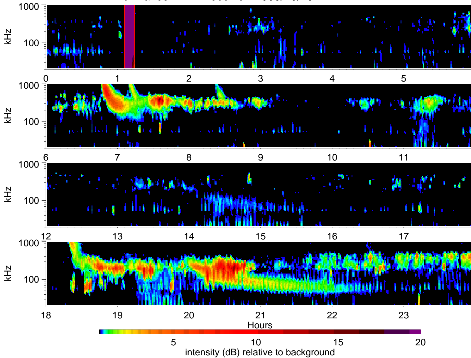
Wind Waves RAD1 receiver: 2005/10/13
