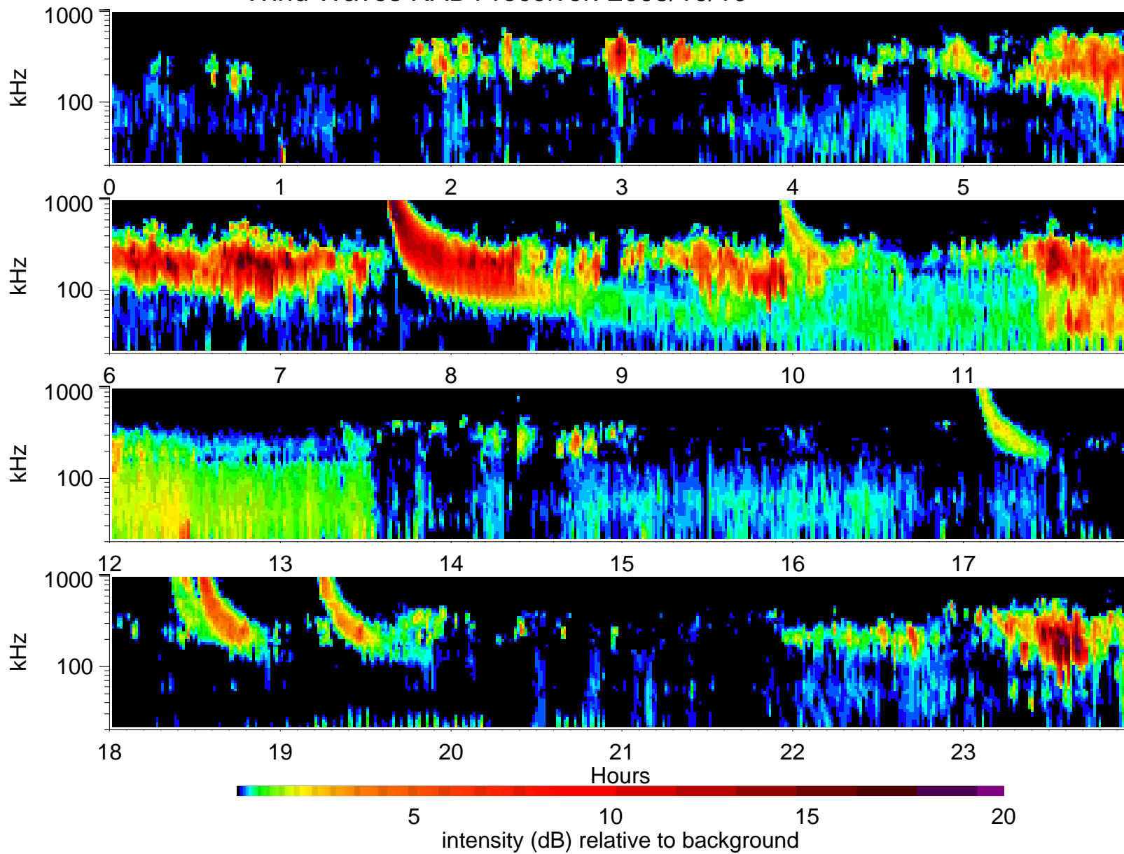
Wind Waves RAD1 receiver: 2005/10/10
