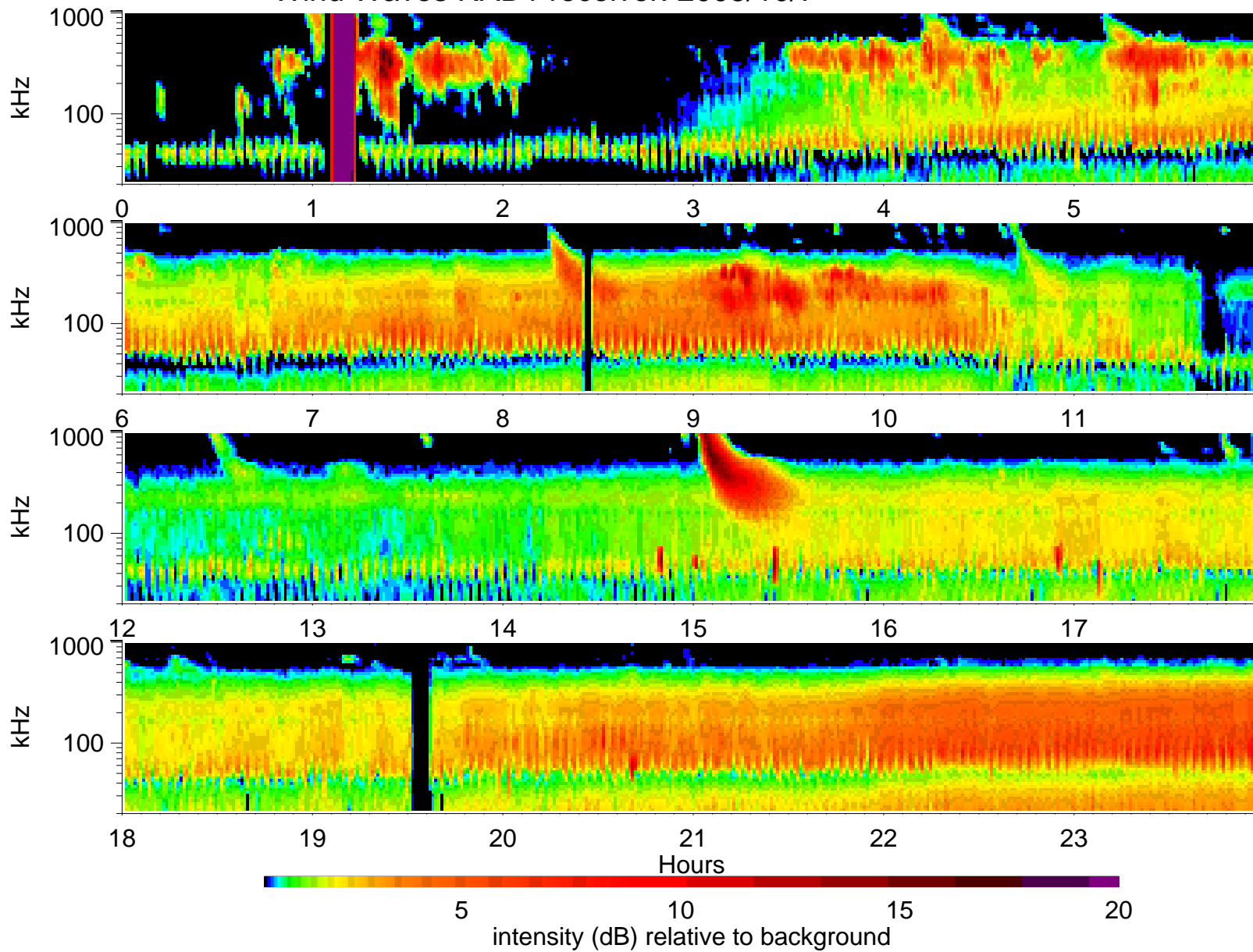
Wind Waves RAD1 receiver: 2005/10/7
