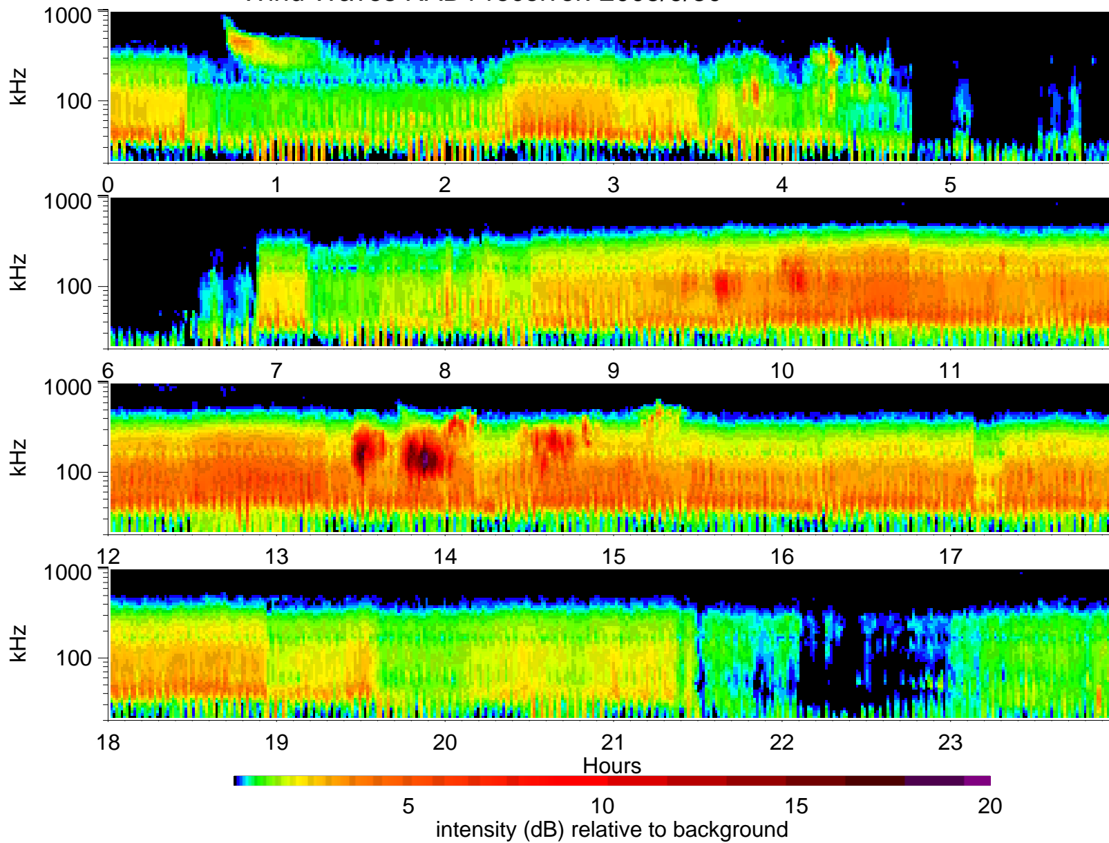
Wind Waves RAD1 receiver: 2005/9/30
