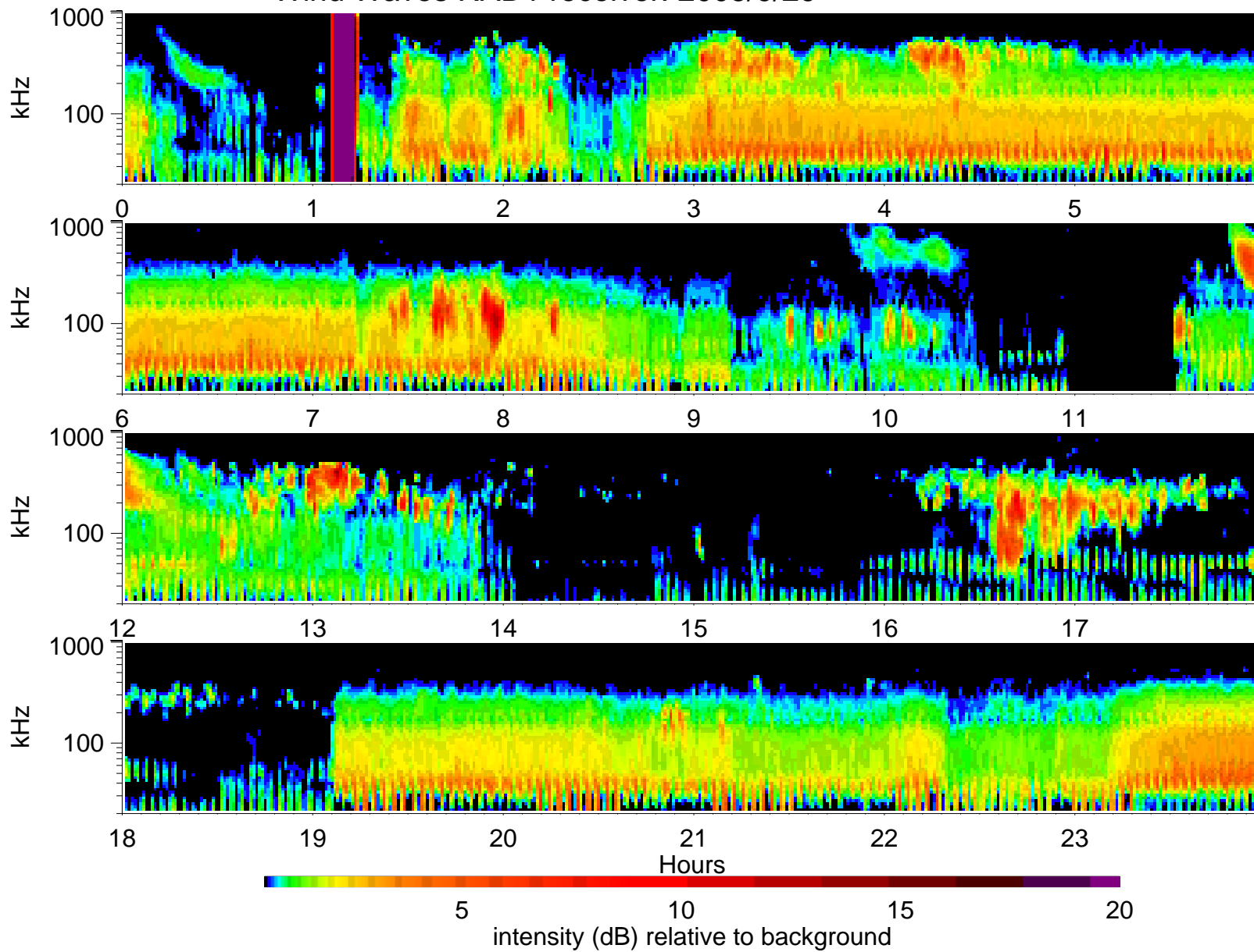
Wind Waves RAD1 receiver: 2005/9/29
