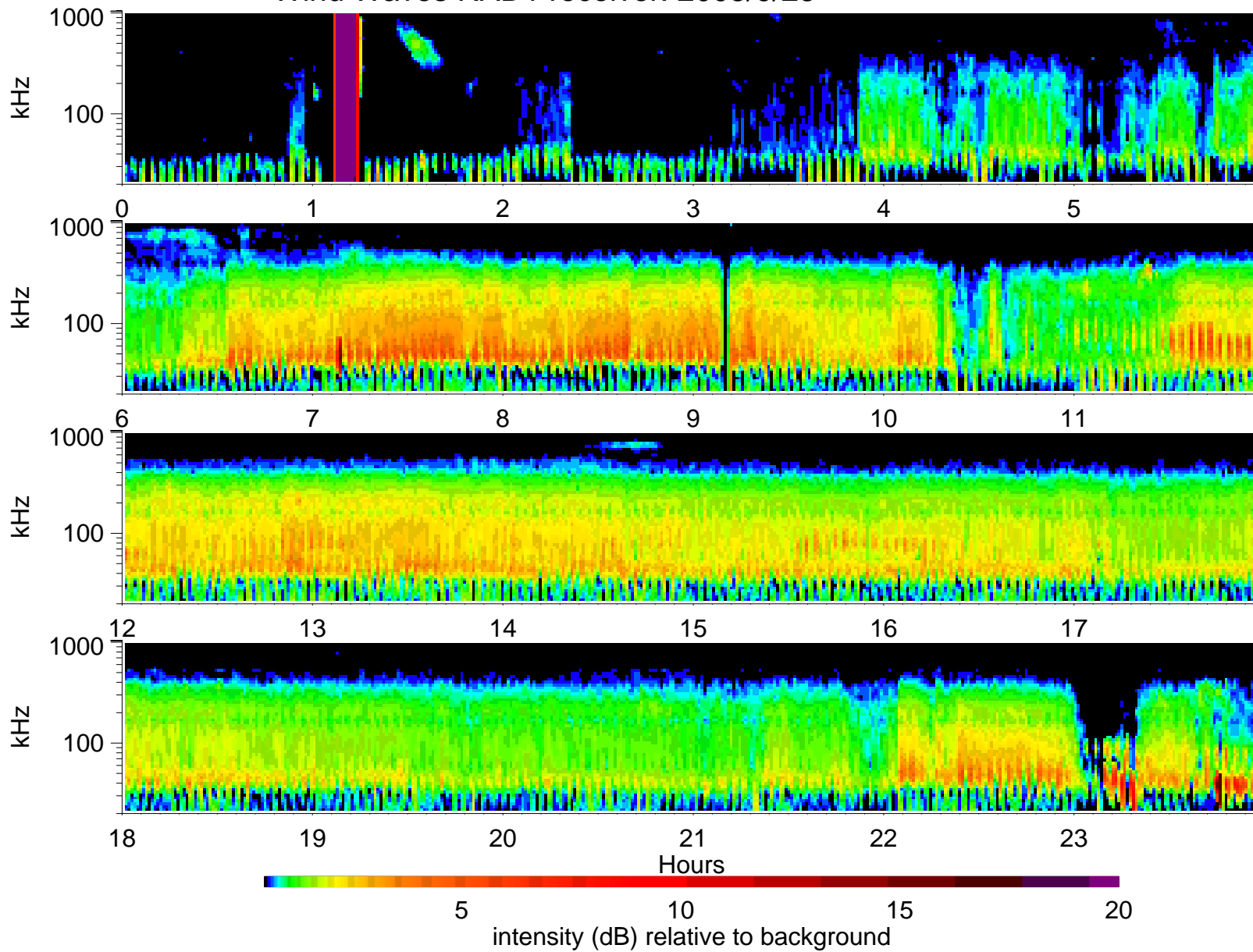
Wind Waves RAD1 receiver: 2005/9/25
