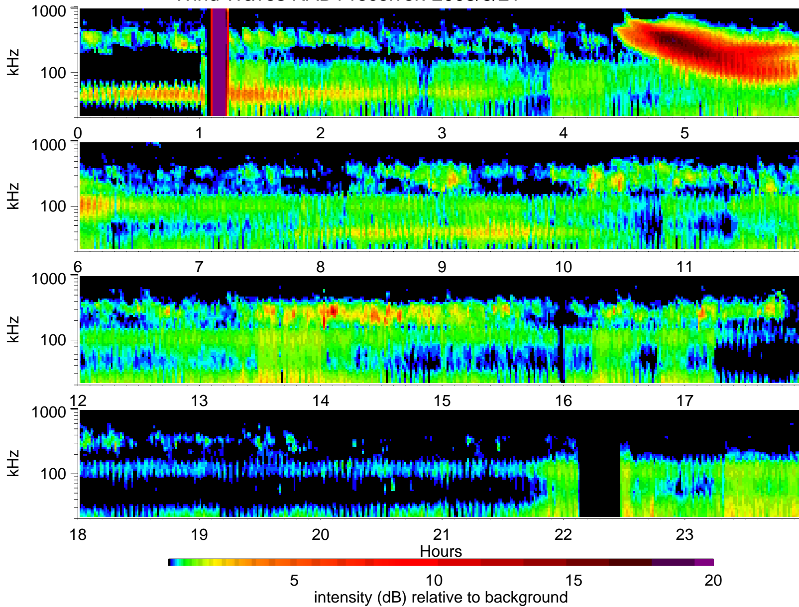
Wind Waves RAD1 receiver: 2005/9/21
