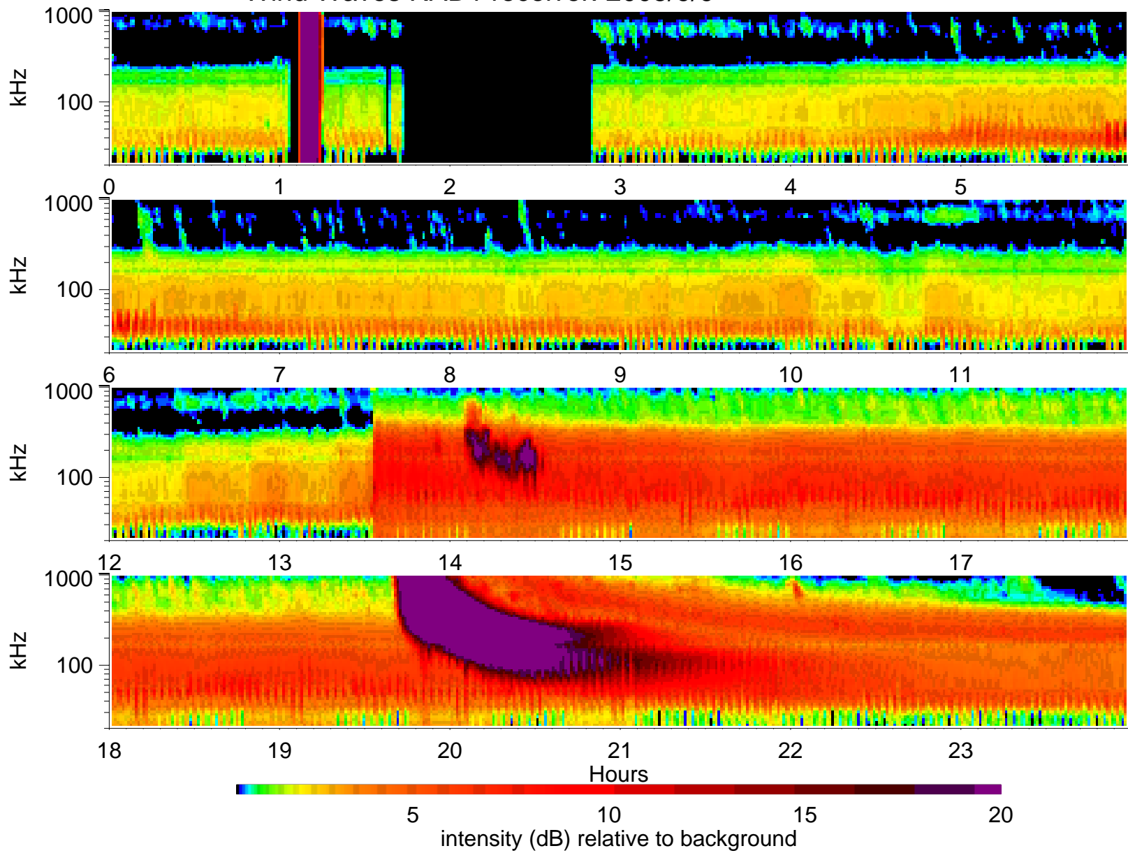
Wind Waves RAD1 receiver: 2005/9/9
