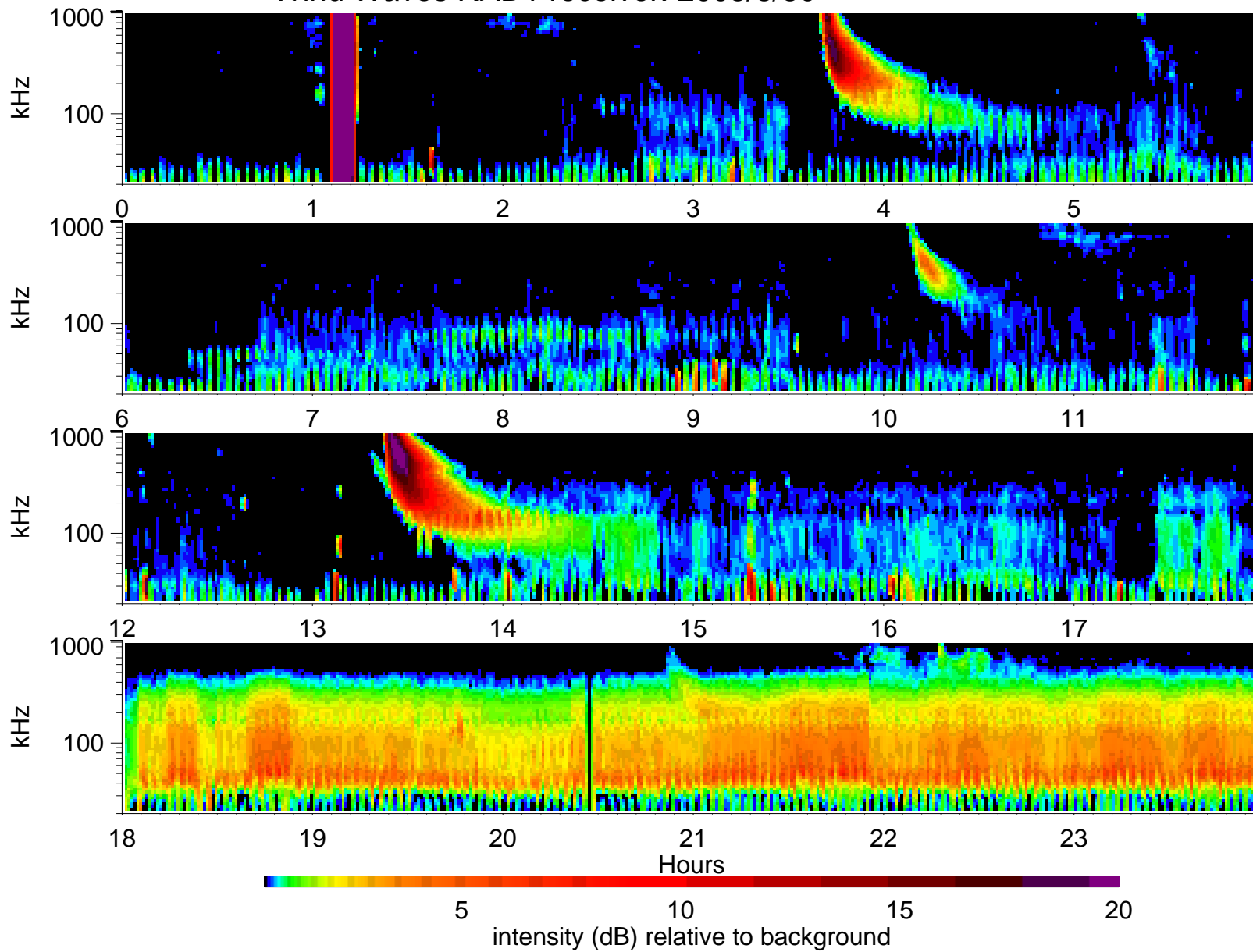
Wind Waves RAD1 receiver: 2005/8/30
