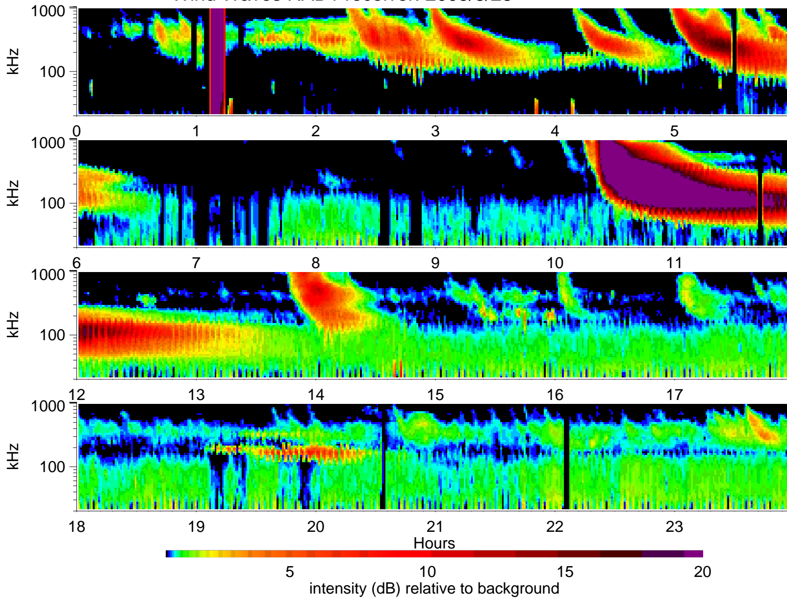
Wind Waves RAD1 receiver: 2005/8/28
