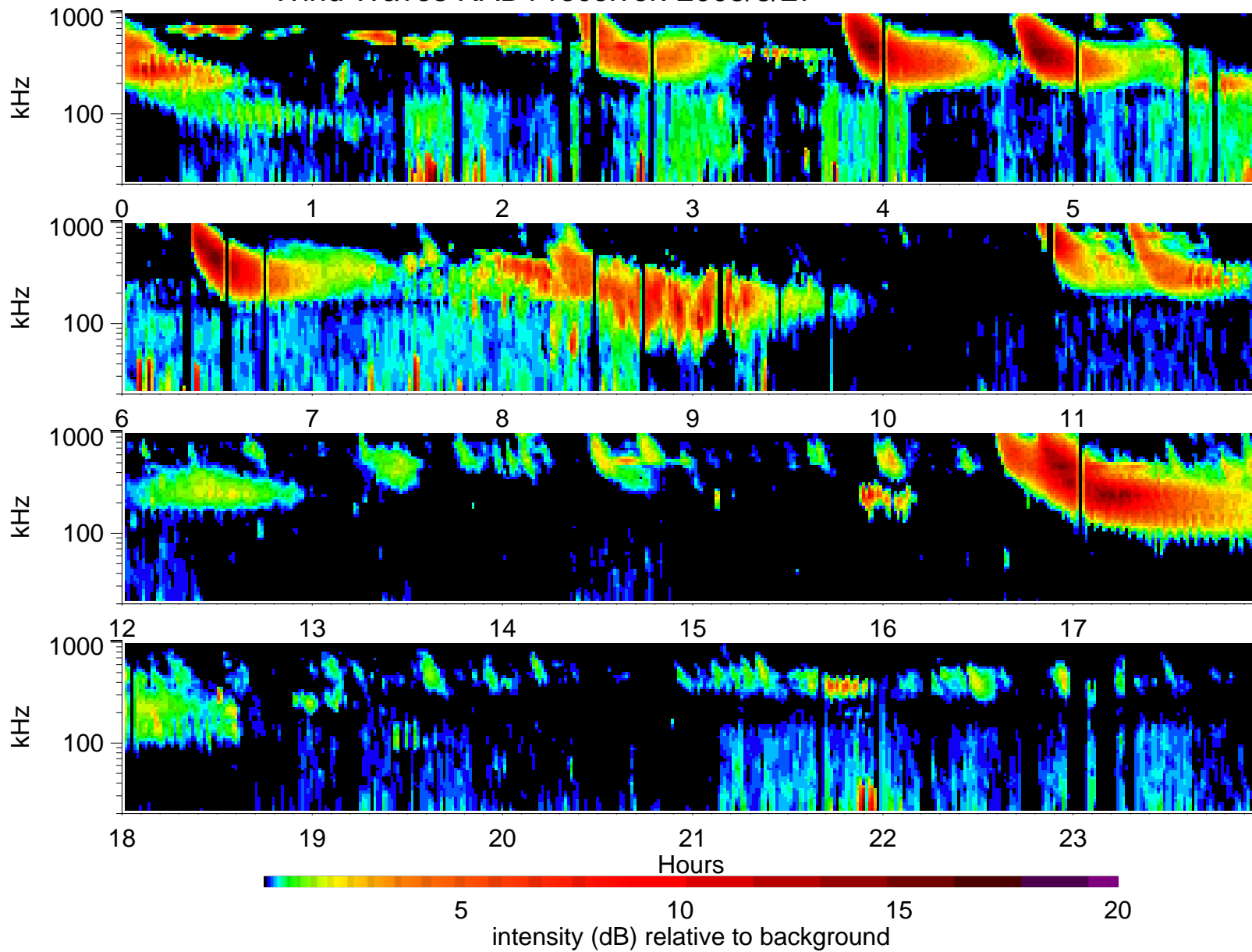
Wind Waves RAD1 receiver: 2005/8/27
