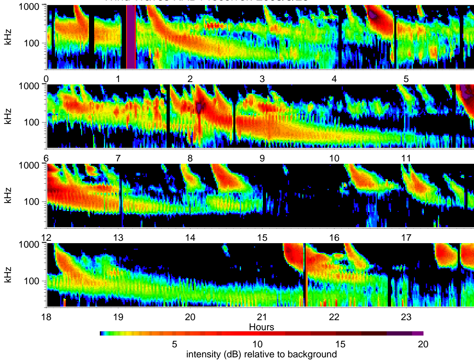
Wind Waves RAD1 receiver: 2005/8/26
