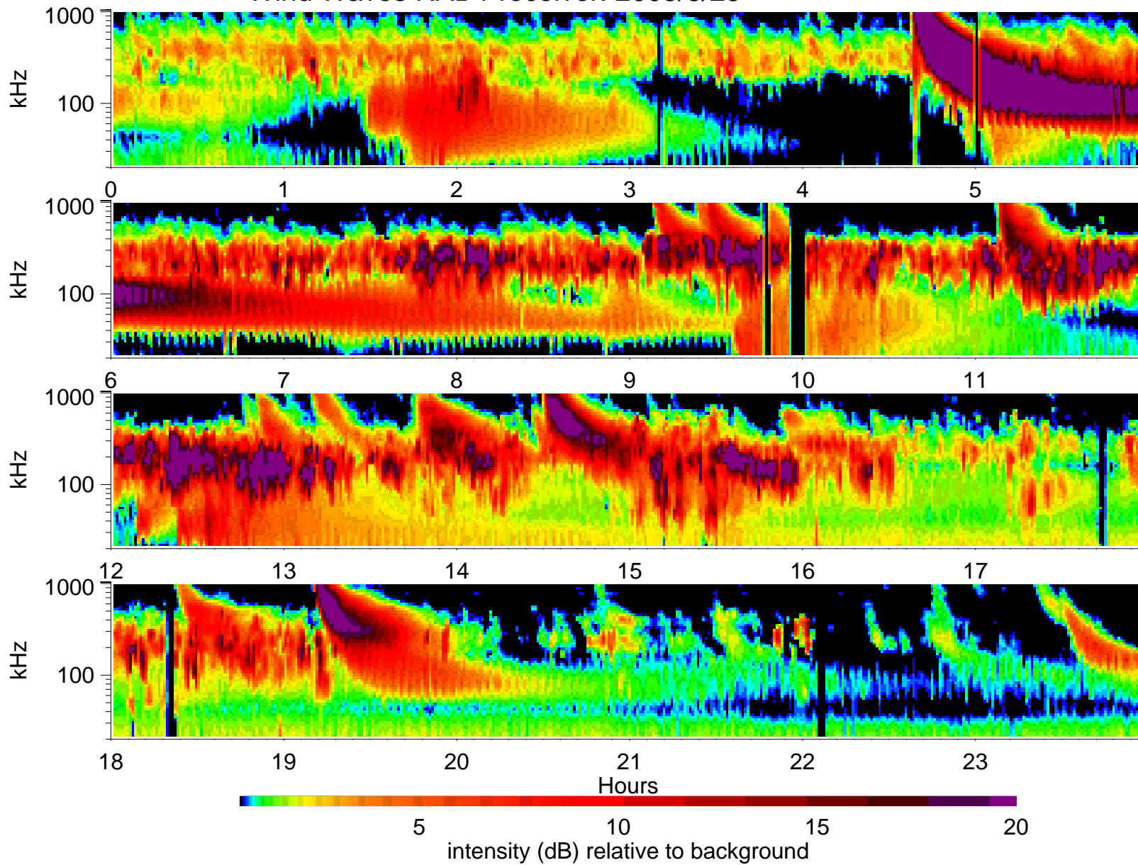
Wind Waves RAD1 receiver: 2005/8/25
