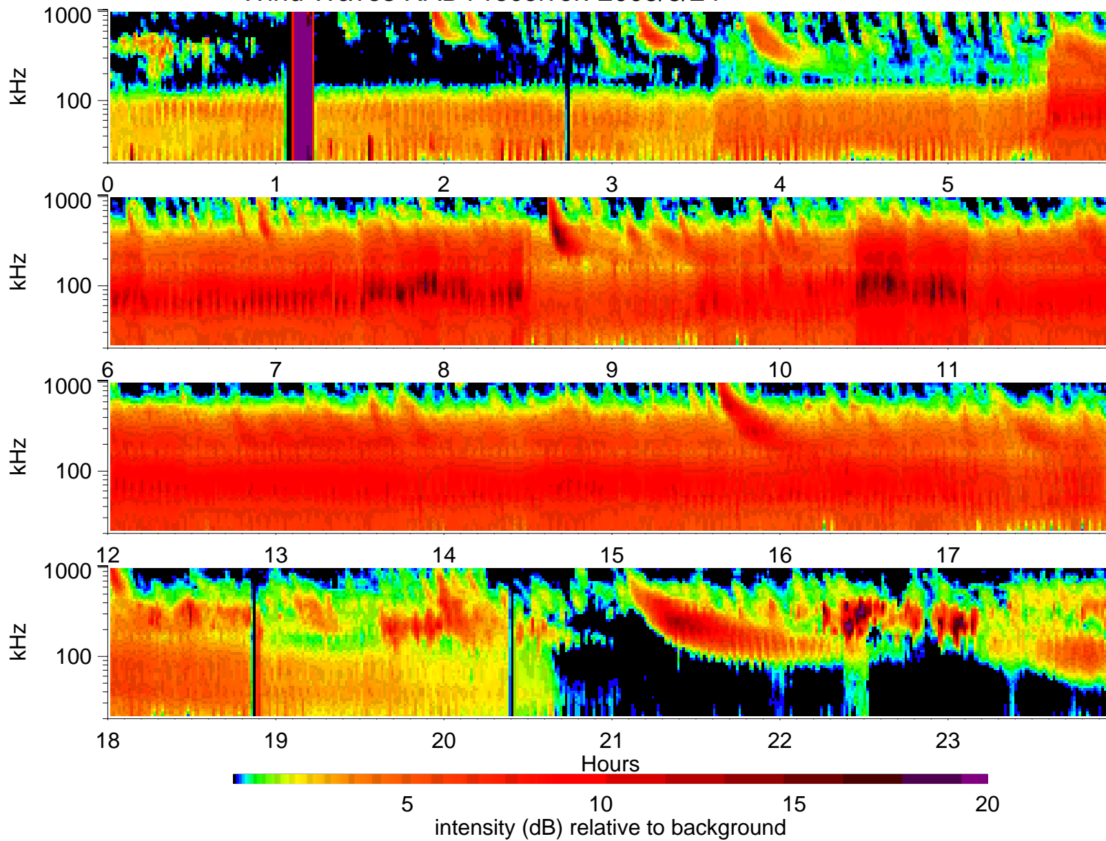
Wind Waves RAD1 receiver: 2005/8/24
