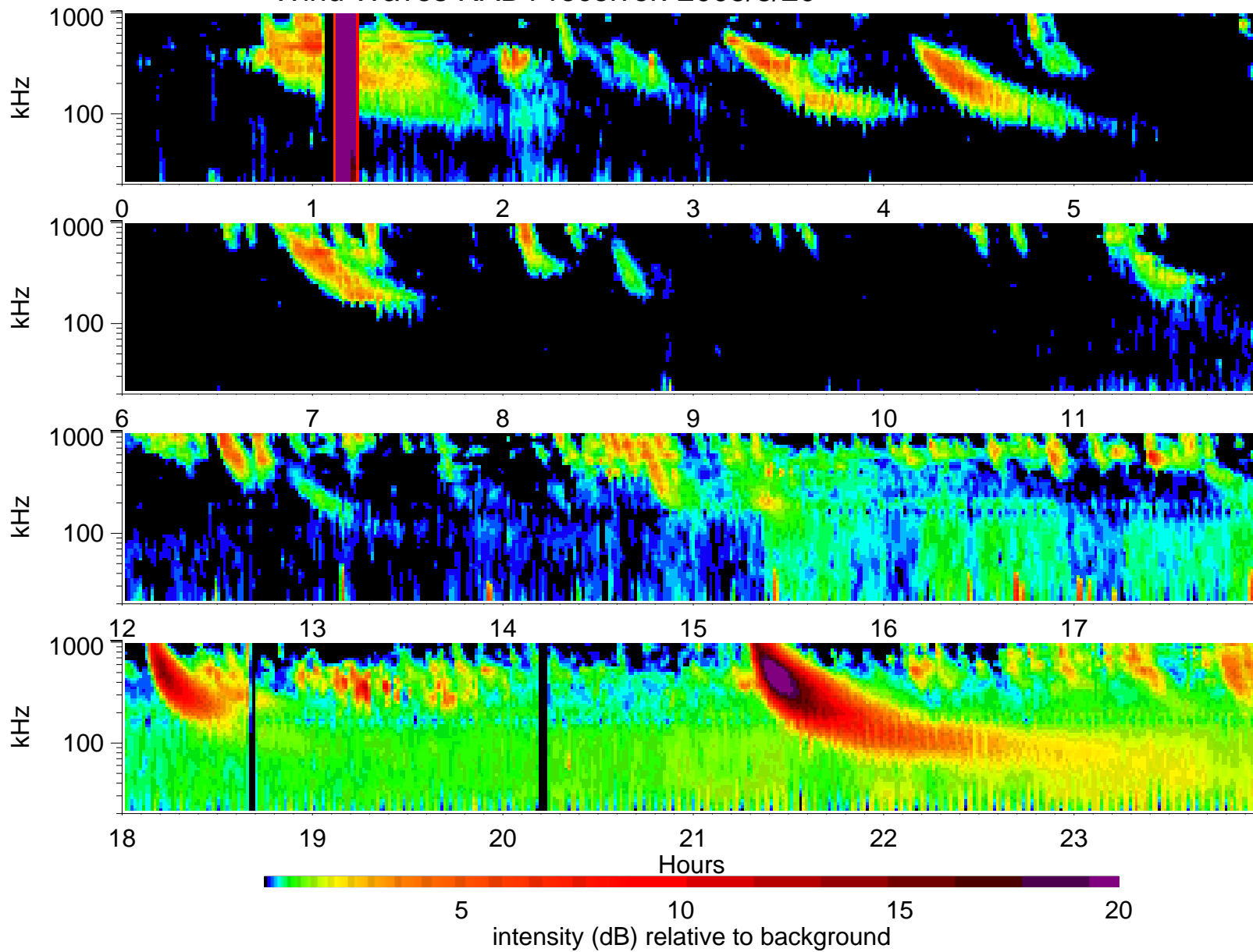
Wind Waves RAD1 receiver: 2005/8/20
