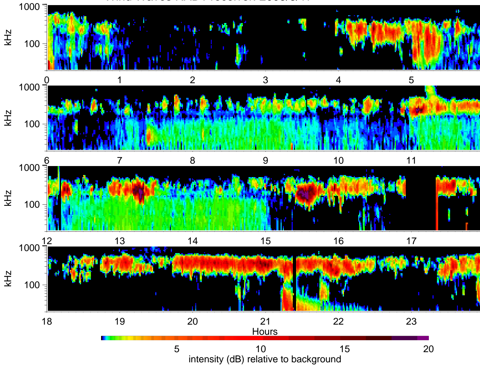
Wind Waves RAD1 receiver: 2005/8/17
