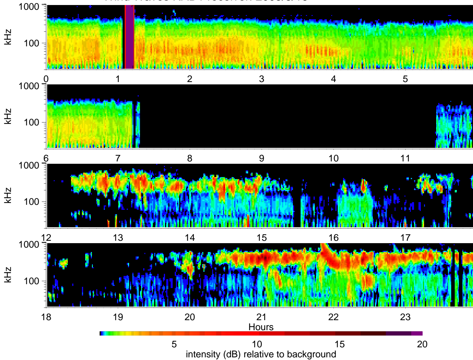
Wind Waves RAD1 receiver: 2005/8/16
