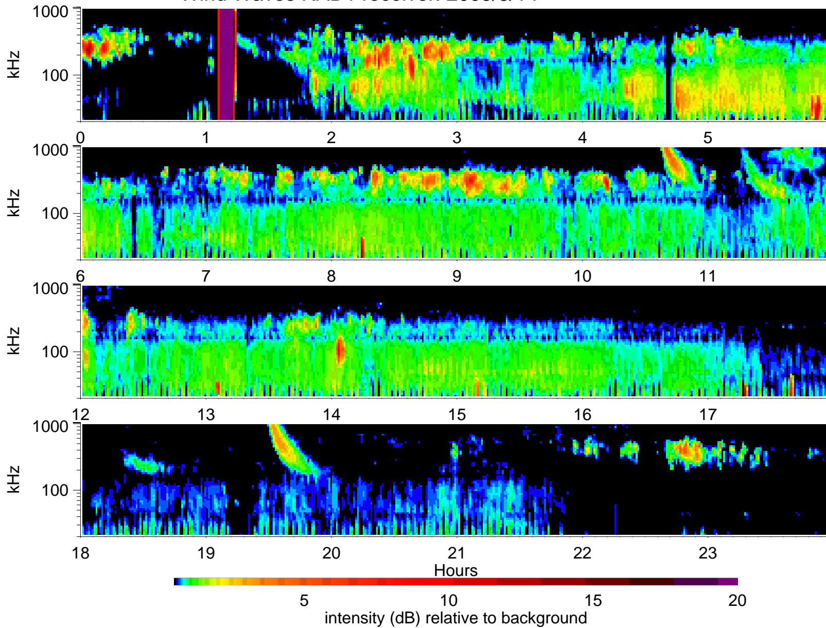
Wind Waves RAD1 receiver: 2005/8/14
