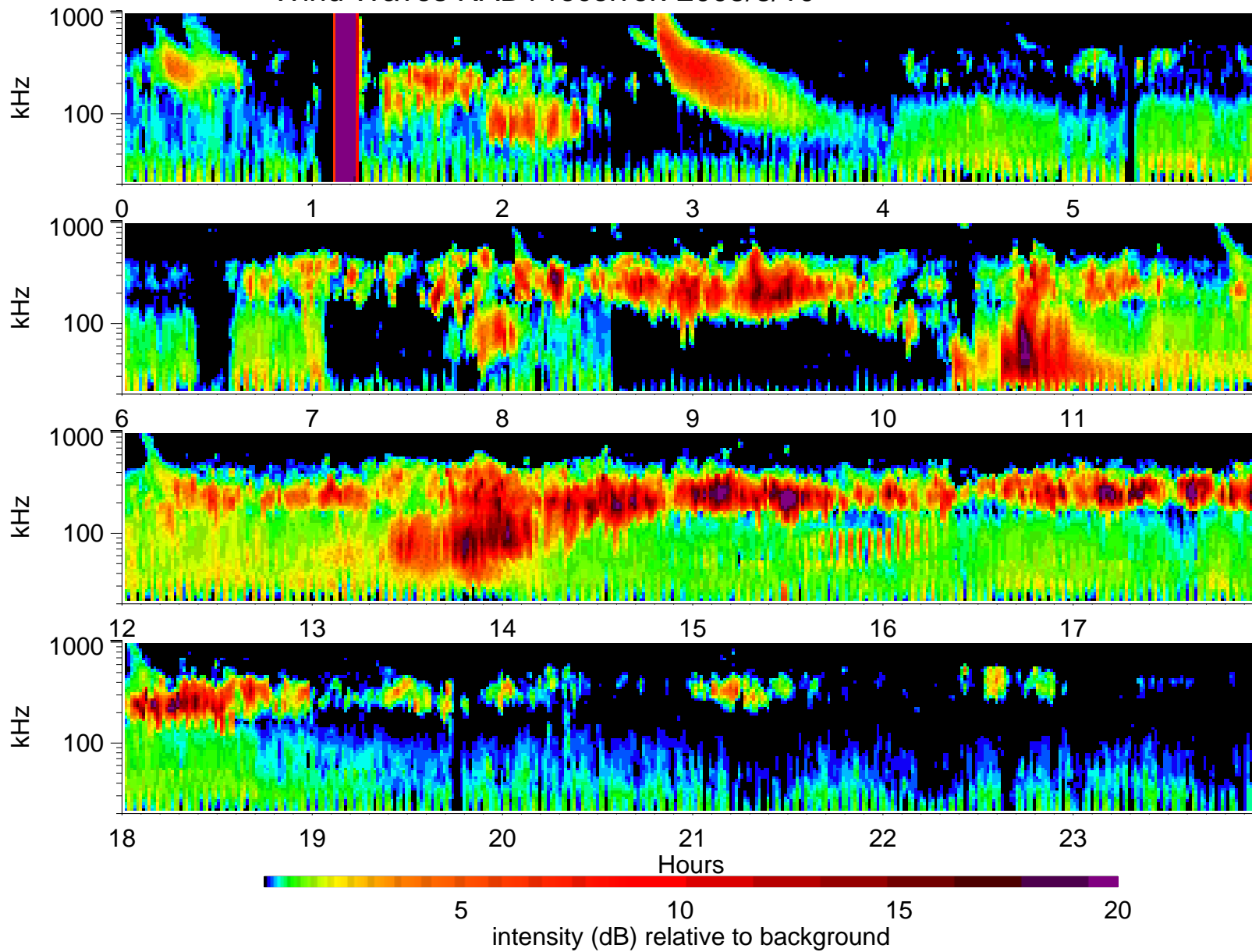
Wind Waves RAD1 receiver: 2005/8/10
