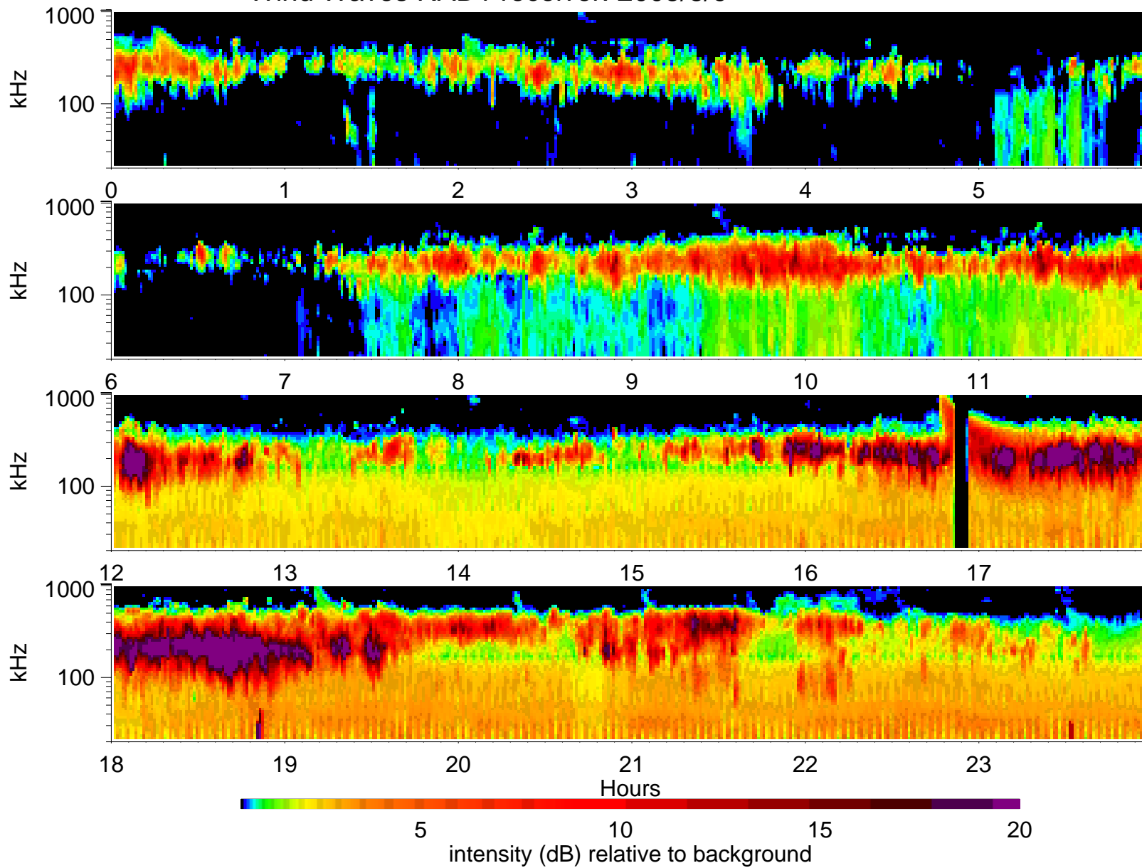
Wind Waves RAD1 receiver: 2005/8/9
