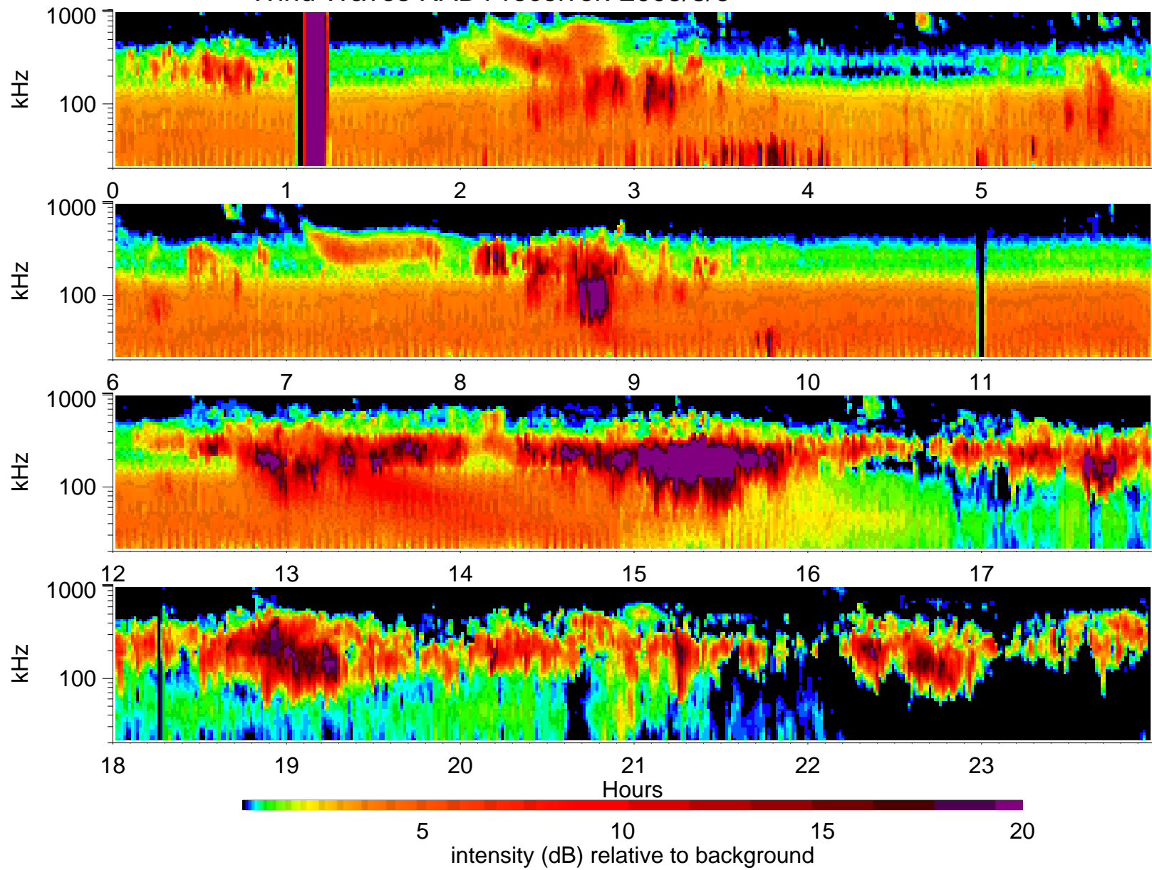
Wind Waves RAD1 receiver: 2005/8/6
