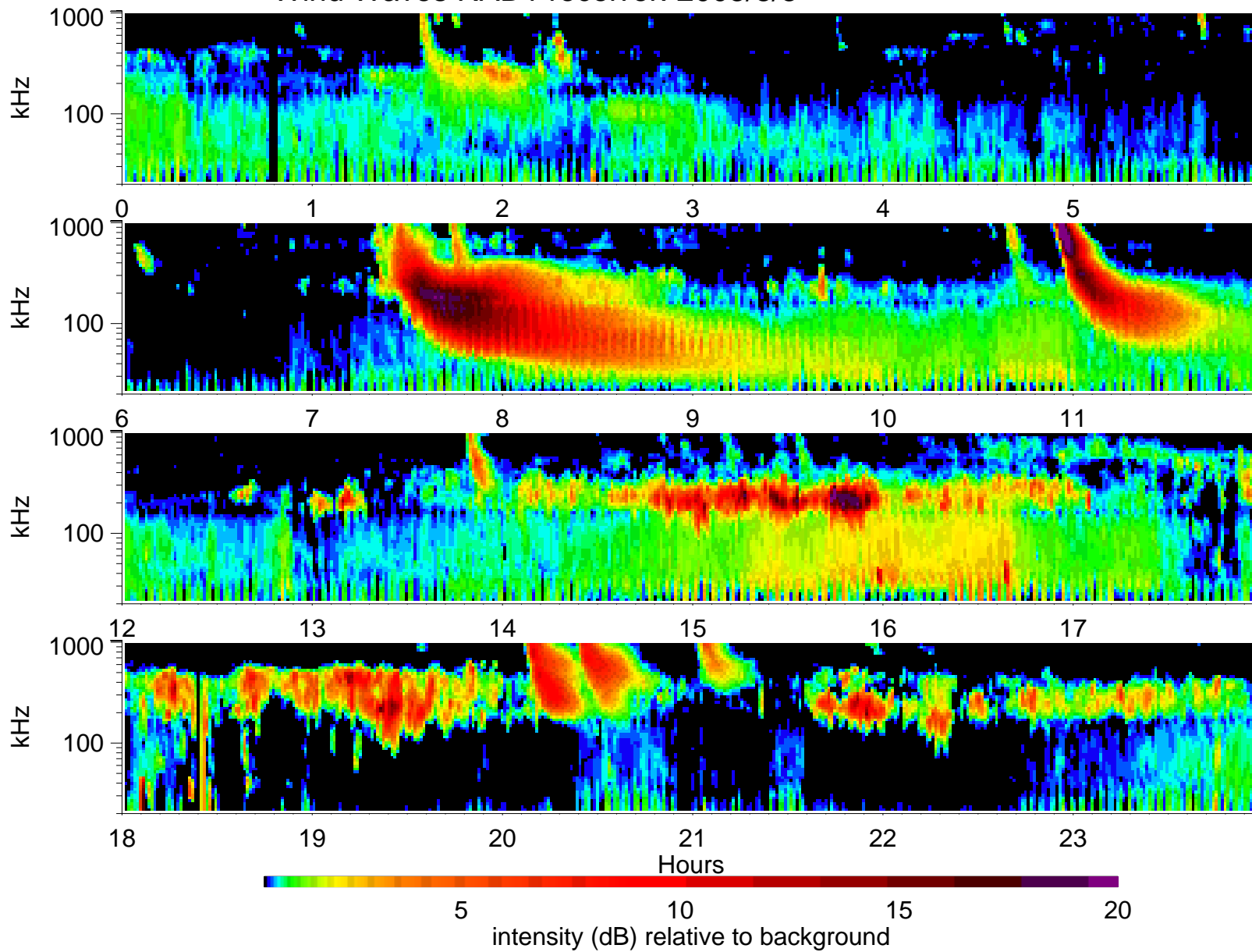
Wind Waves RAD1 receiver: 2005/8/5
