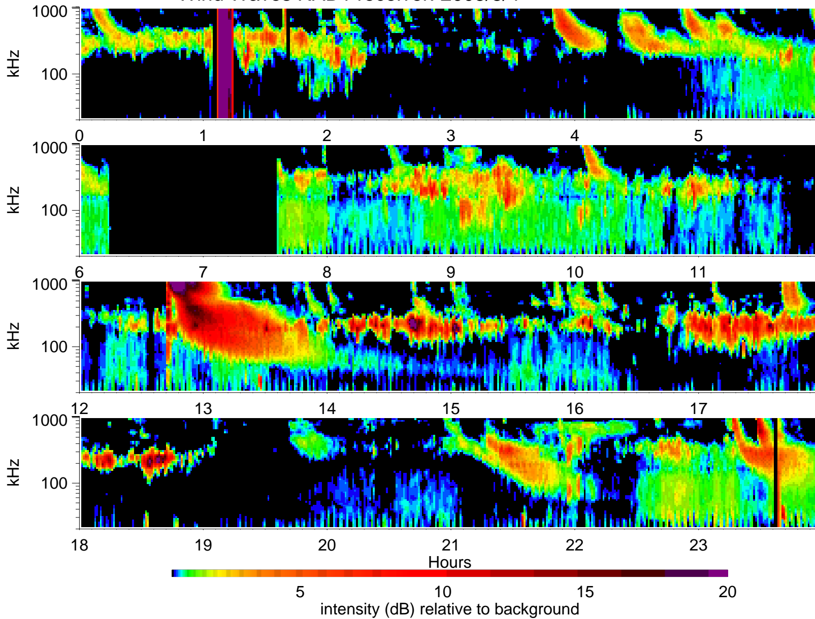
Wind Waves RAD1 receiver: 2005/8/4
