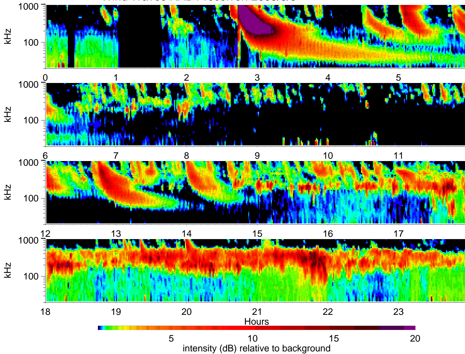
Wind Waves RAD1 receiver: 2005/8/3
