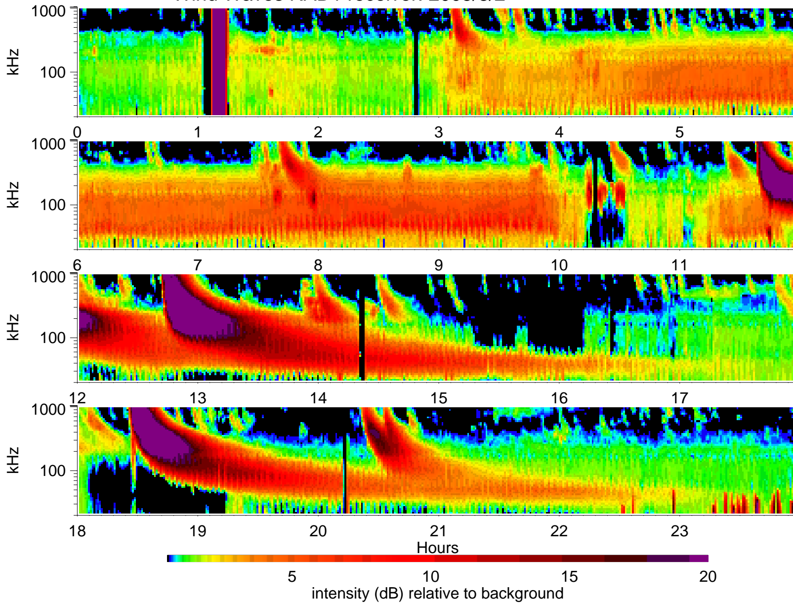
Wind Waves RAD1 receiver: 2005/8/2
