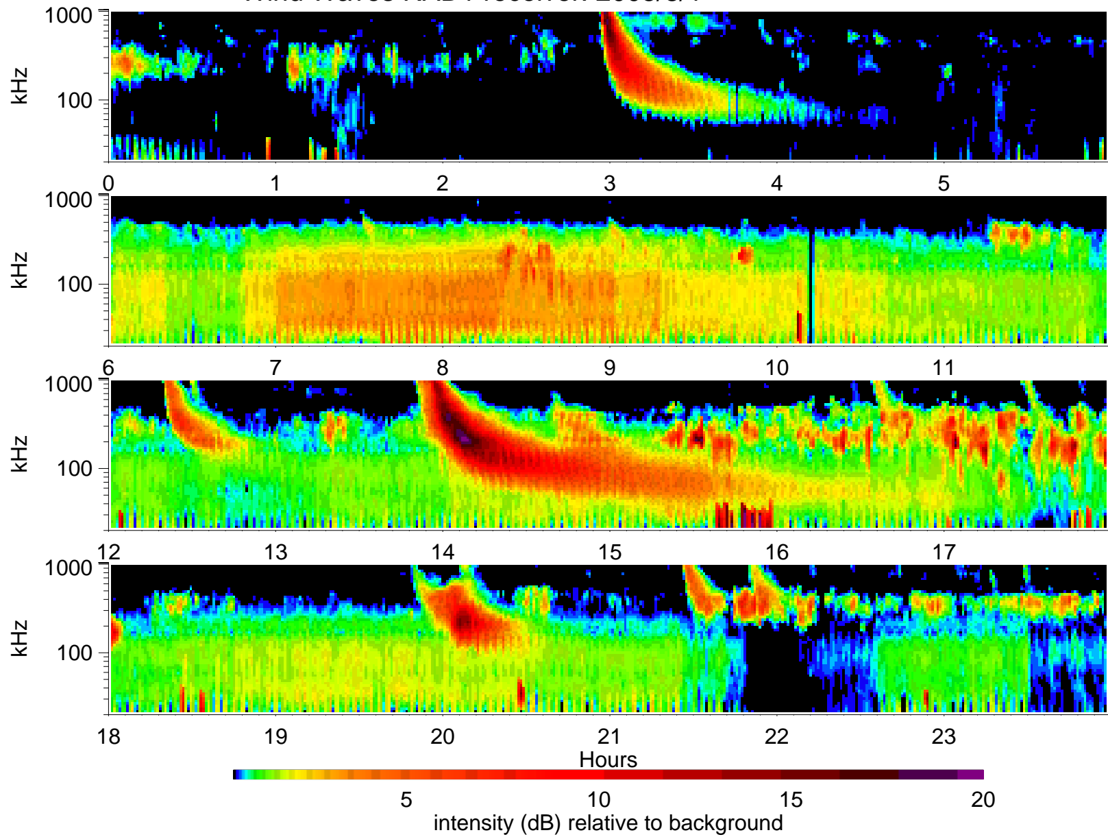
Wind Waves RAD1 receiver: 2005/8/1
